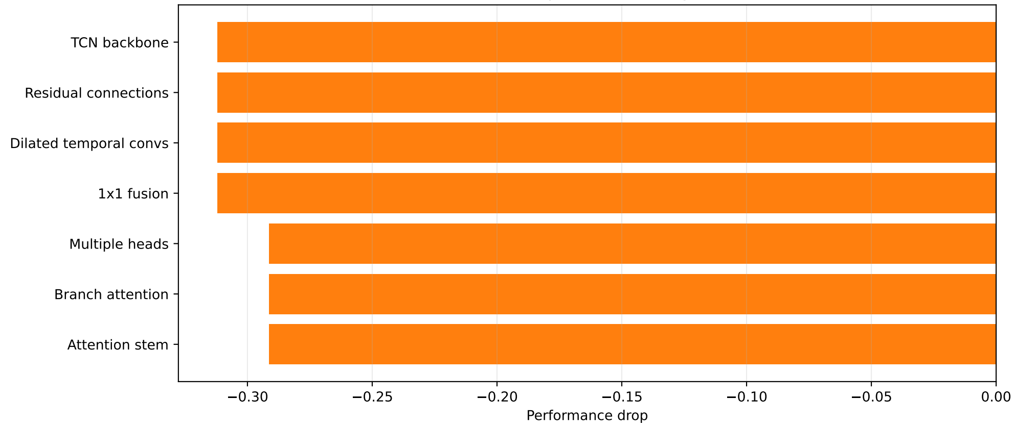
Macro correlation drop when removing each module
