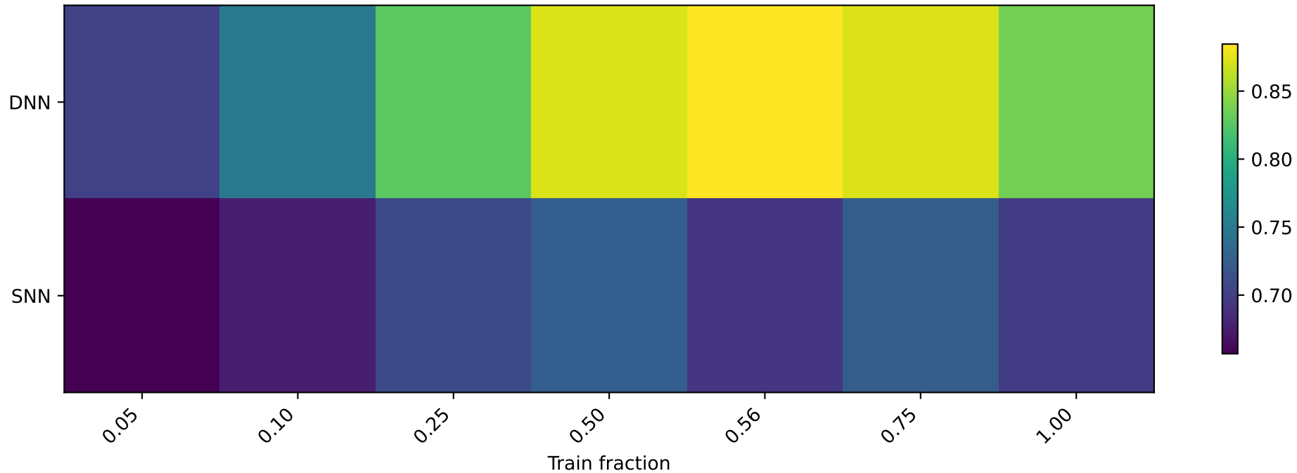
Model-type performance heatmap across train fraction
