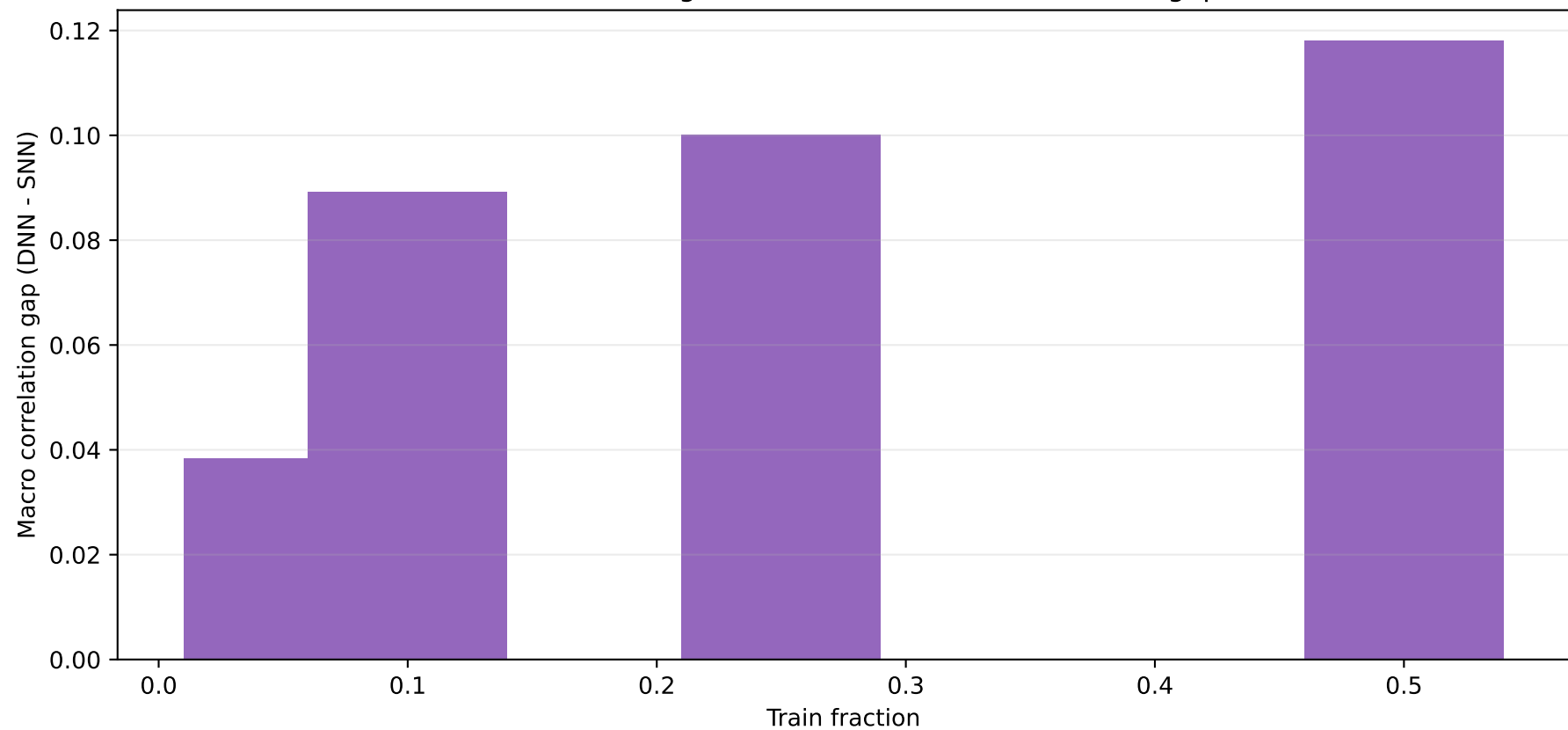
Data-limited regime: DNN-SNN macro correlation gap
