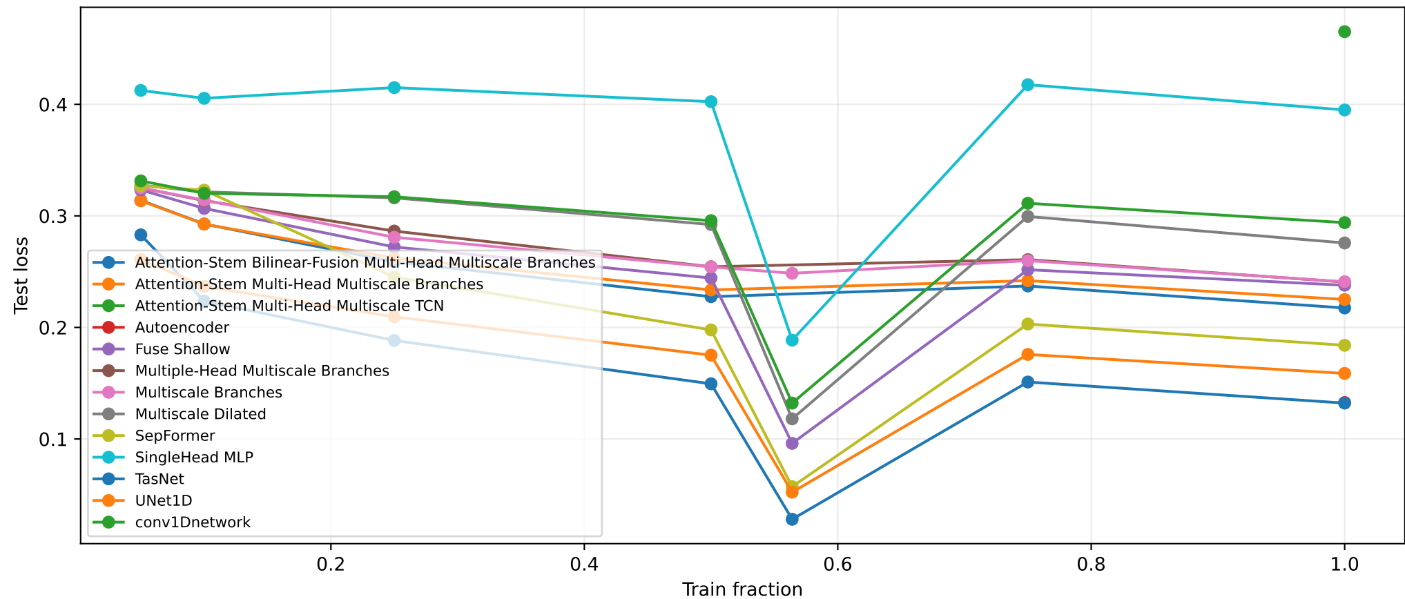
Test loss vs train fraction
