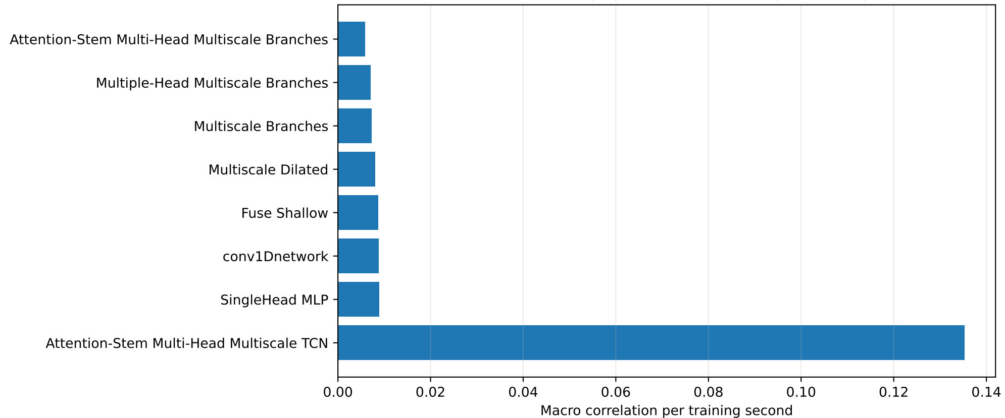
Cost-normalized ranking by macro correlation per training second
