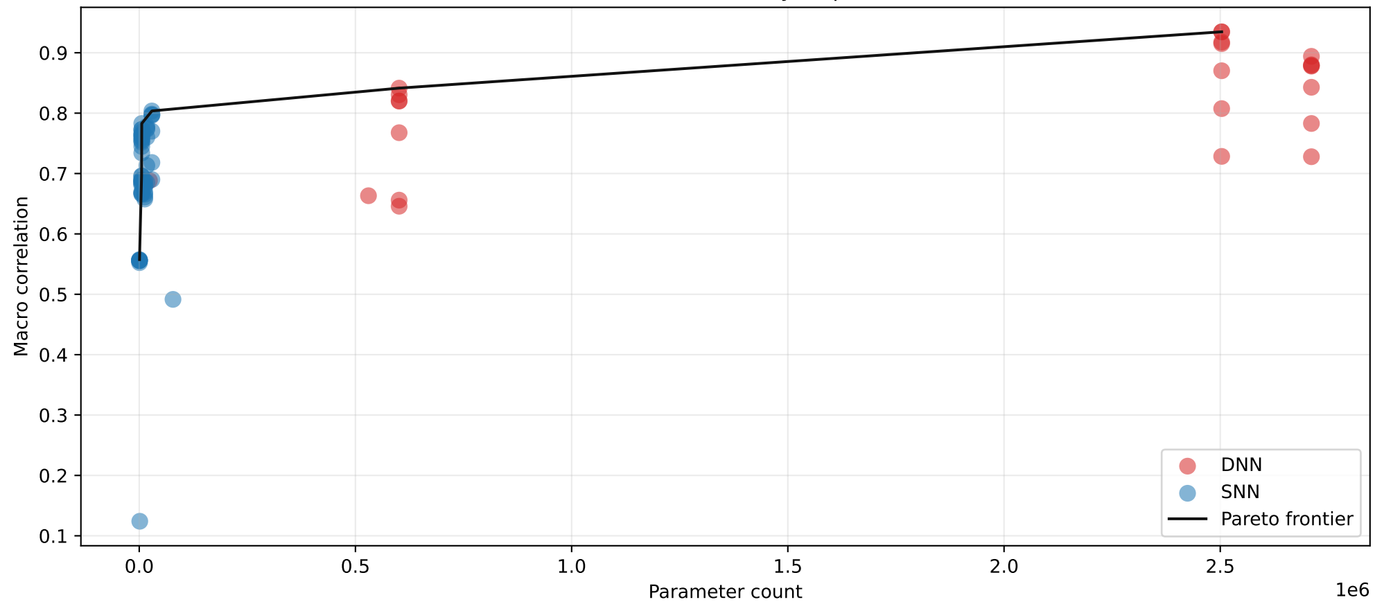
Pareto frontier for accuracy vs parameters
