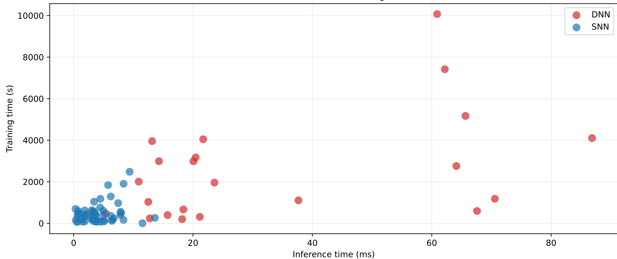
Inference time vs training time
