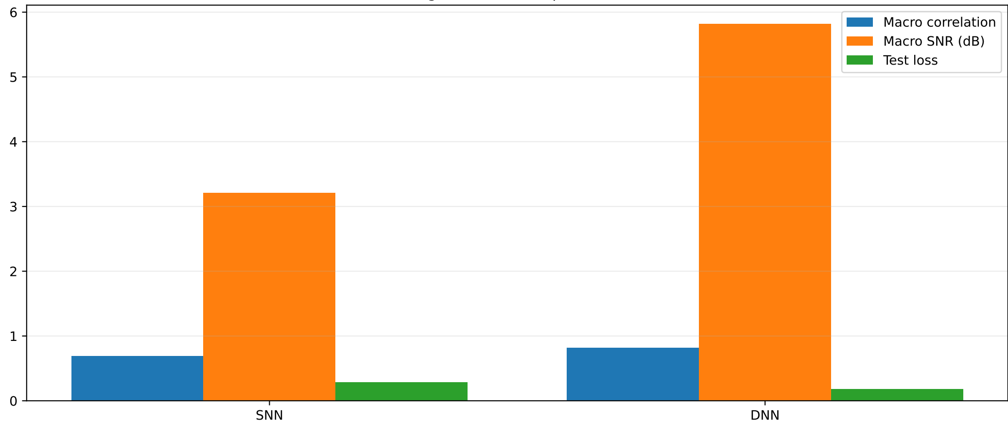
Average SNN vs DNN performance
