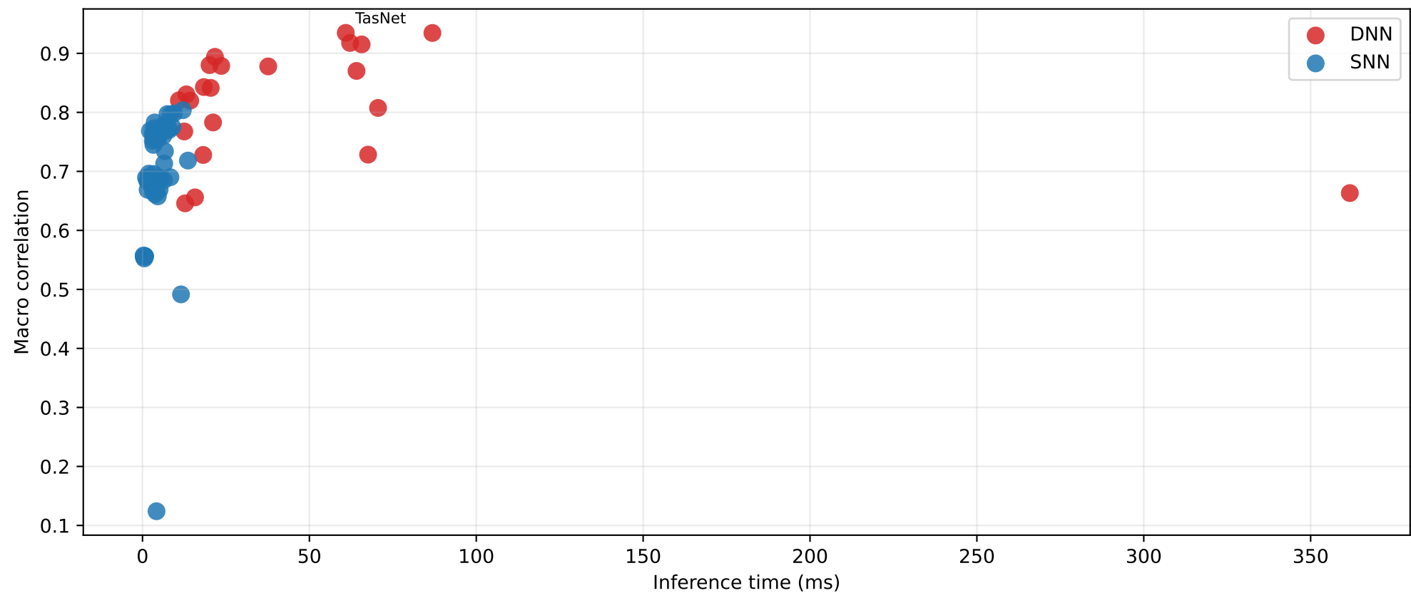
Macro correlation vs inference time
