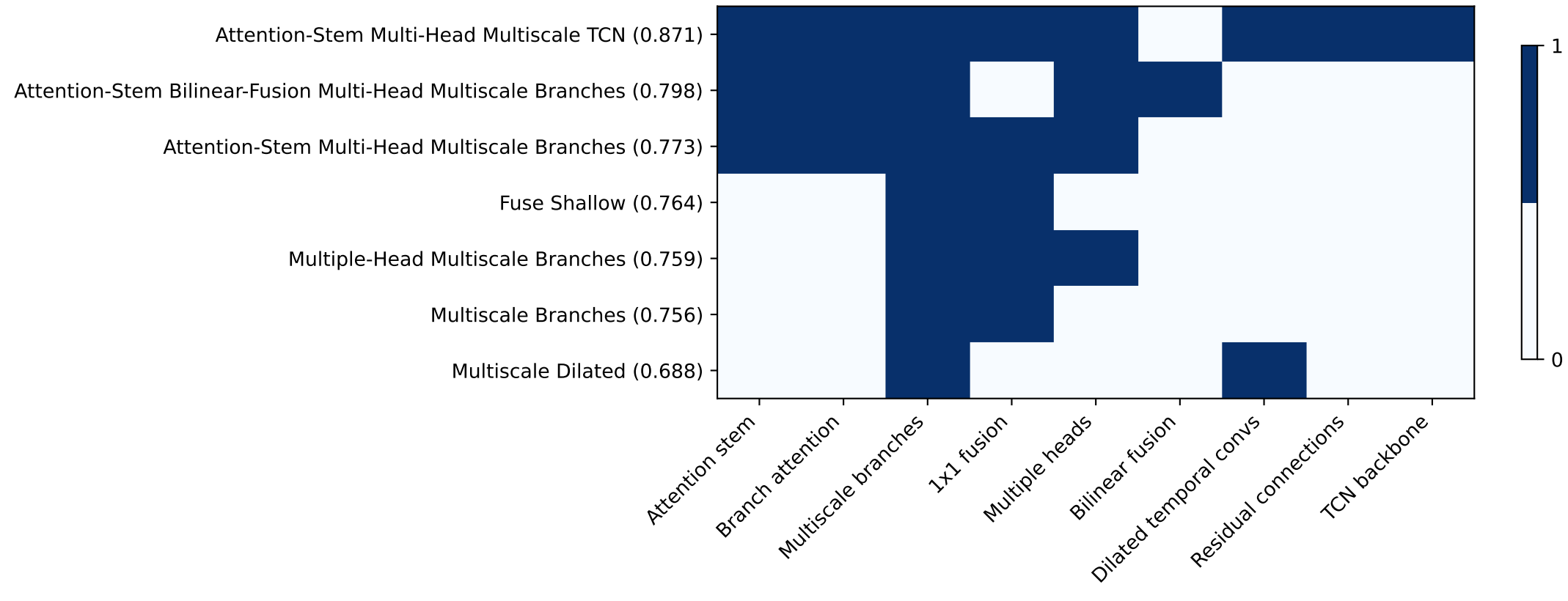
Enabled modules vs Macro correlation
