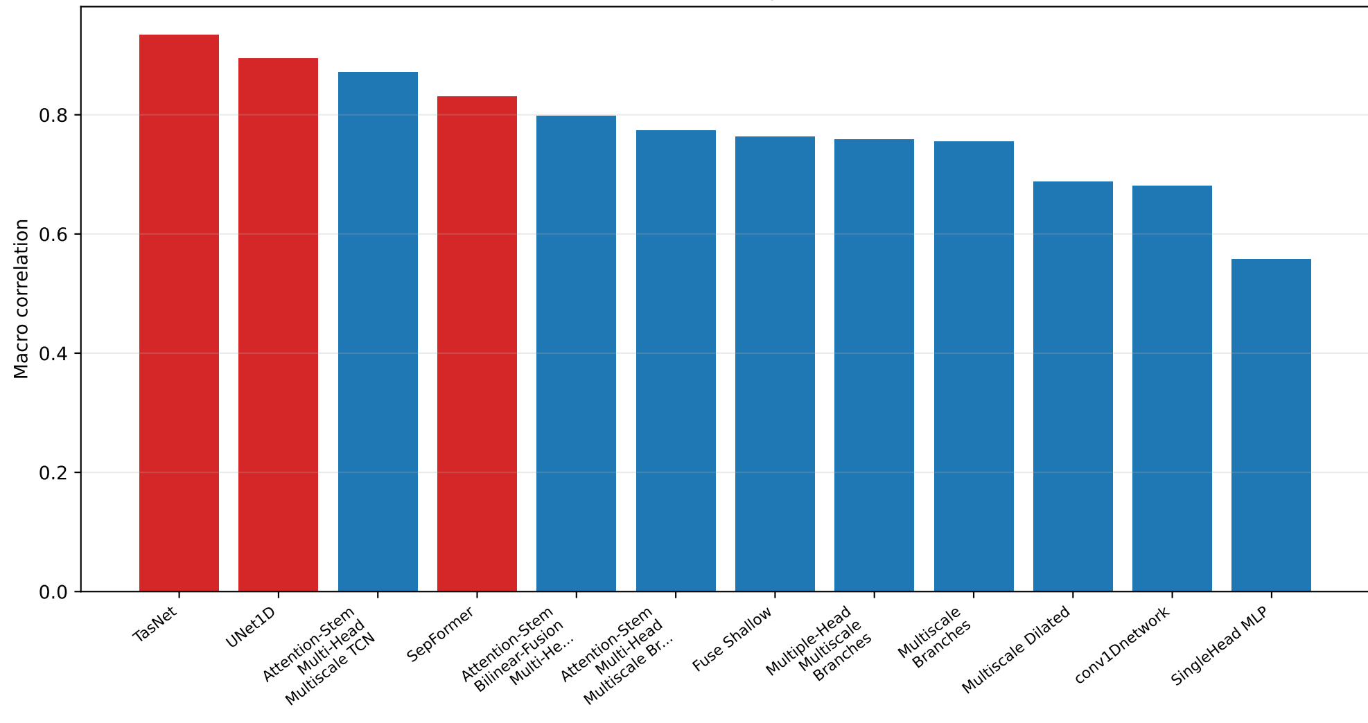
Macro correlation per model
