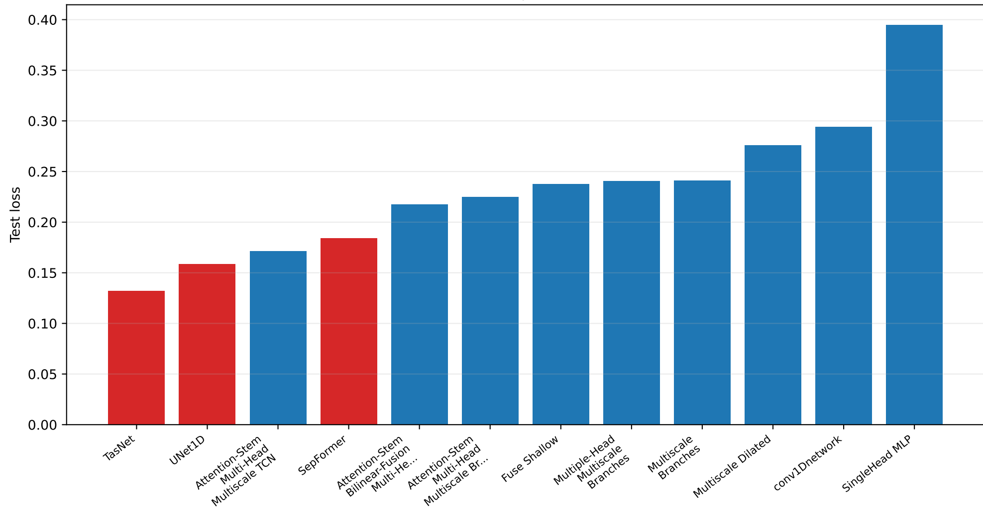
Test loss per model
