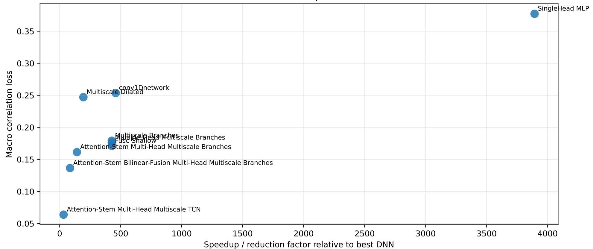
Parameter reduction vs performance loss
