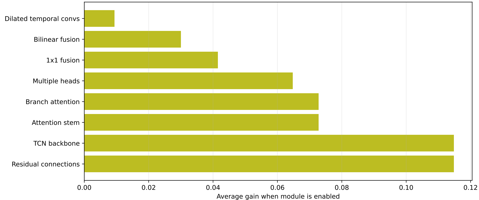
Selected modifications ranked by macro correlation gain
