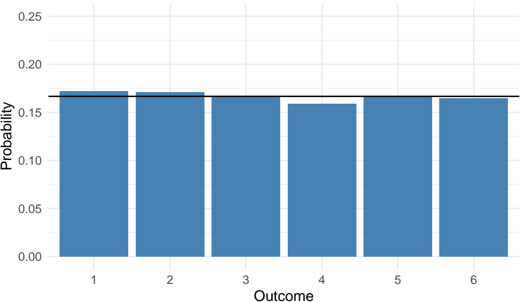
Rolling a die 10000 times ( k = 6 , p = 1/6 )
