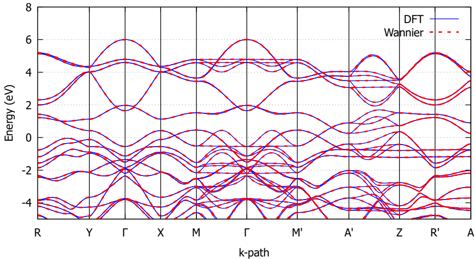
RuO 2 Band Structure
