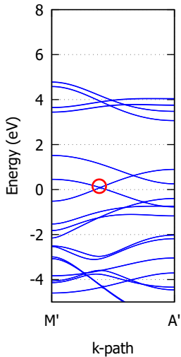
RuO 2 Band Structure
