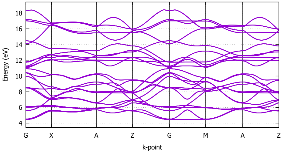
Band structure of RuO 2
