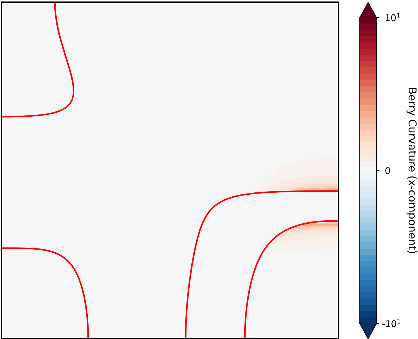
RuO2 K-slice Berry Curvature (x-component) with Fermi Lines
