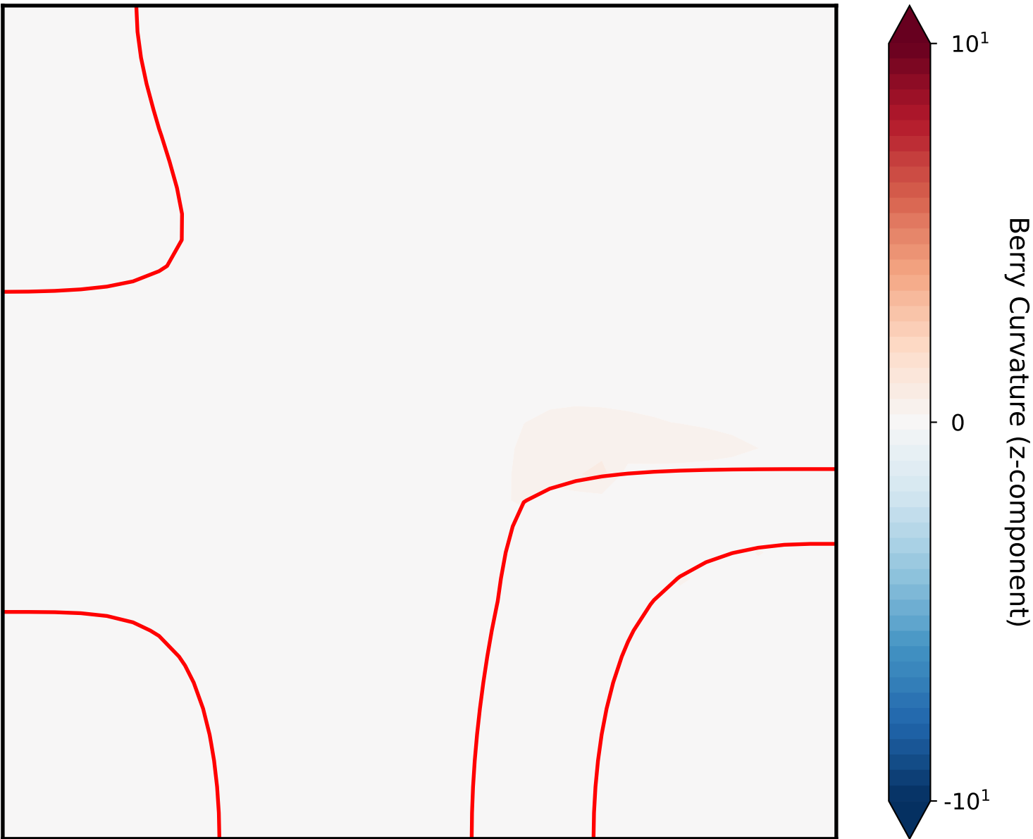
RuO2 K-slice Berry Curvature (z-component) with Fermi Lines
