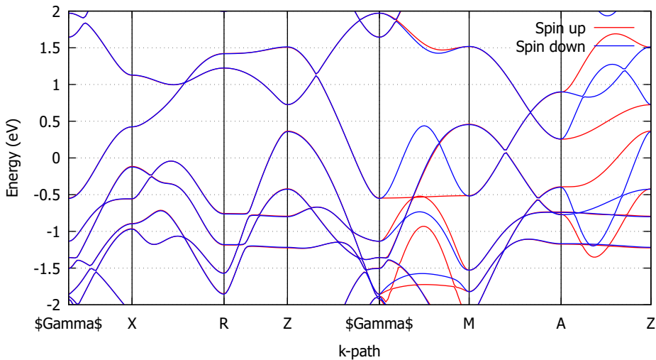
\text{RuO}_2 Band Structure (Spin-Resolved)
