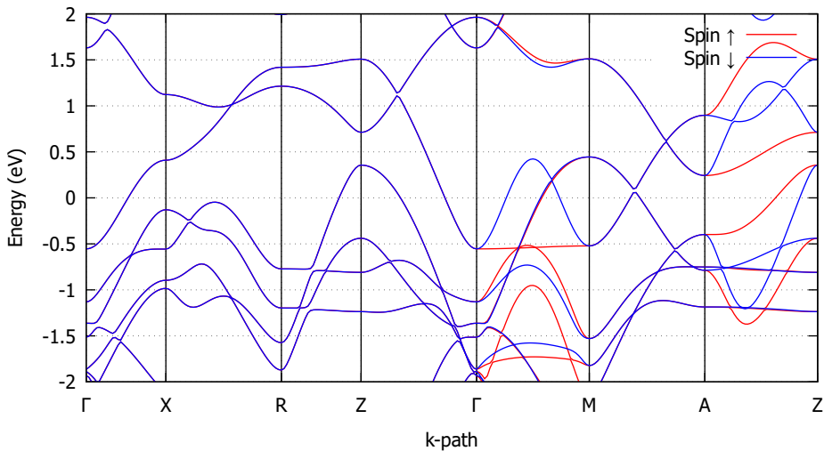
RuO 2 Band Structure (Spin-Resolved)
