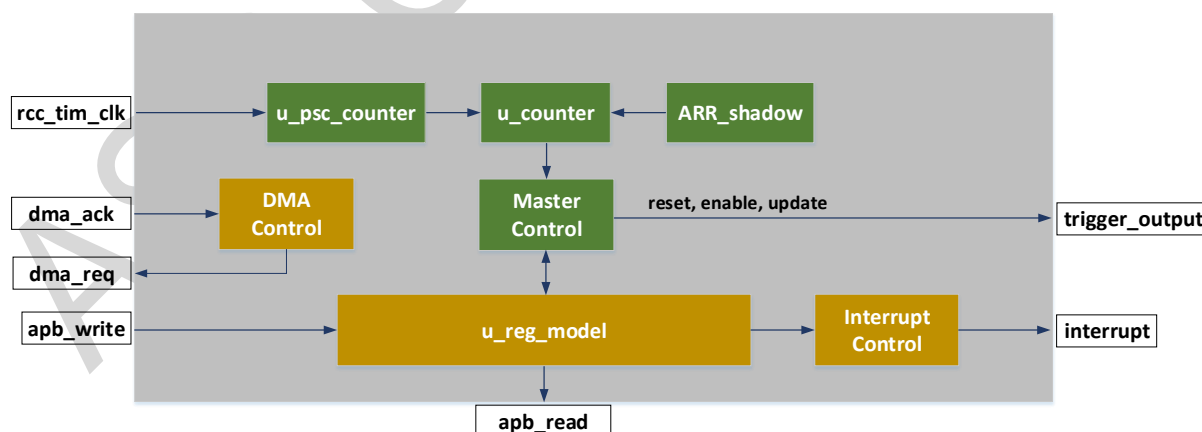
Figure 17-1 BSTIMER Diagram
