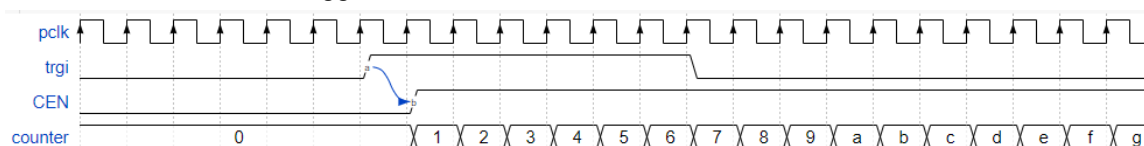
Figure 22-18 Trigger mode waveform in slave mode
