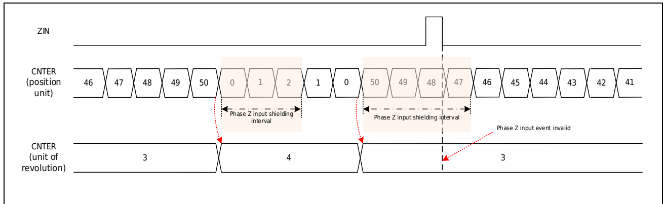
Figure 17-25 Revolution counting mode - Mixed counting Z-phase shielding action example 2
