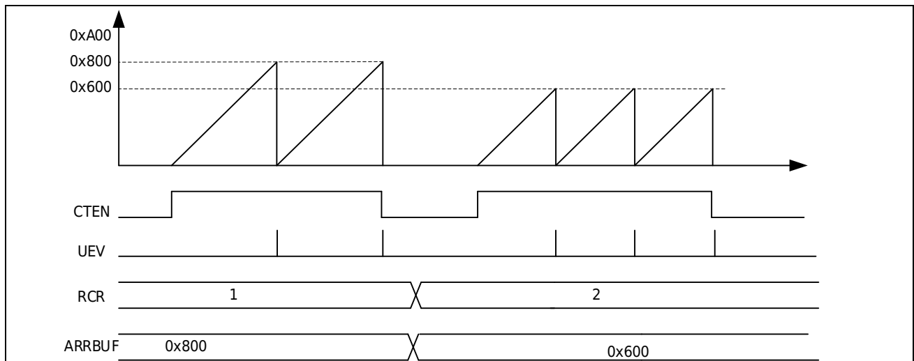
Figure 14-44 Counting Single Pulse Mode on Ramp Waveform
