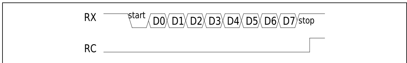
Figure 22-5 Mode1 receiving data
