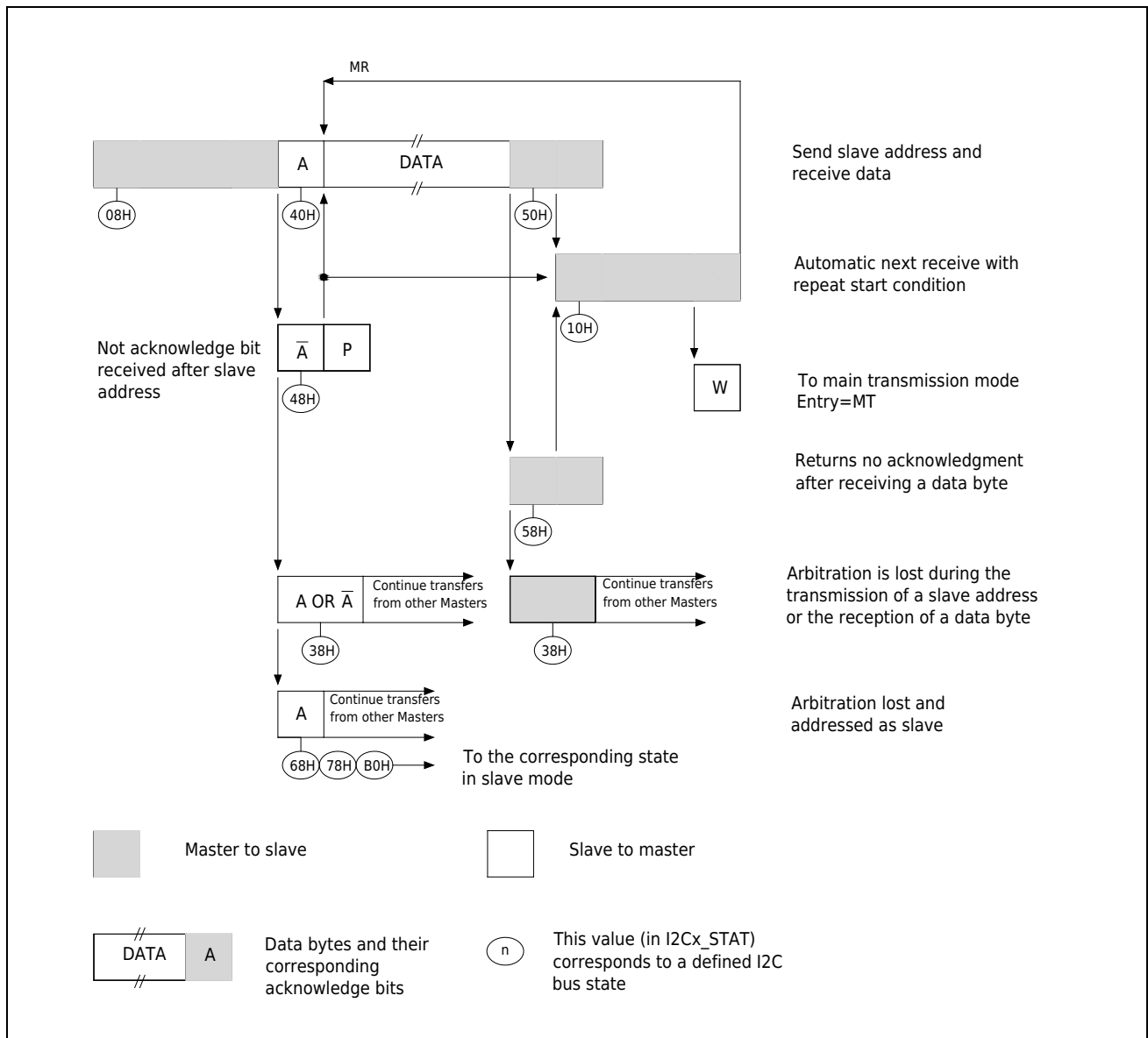
Figure 7-10 I2C master receiving state diagram
