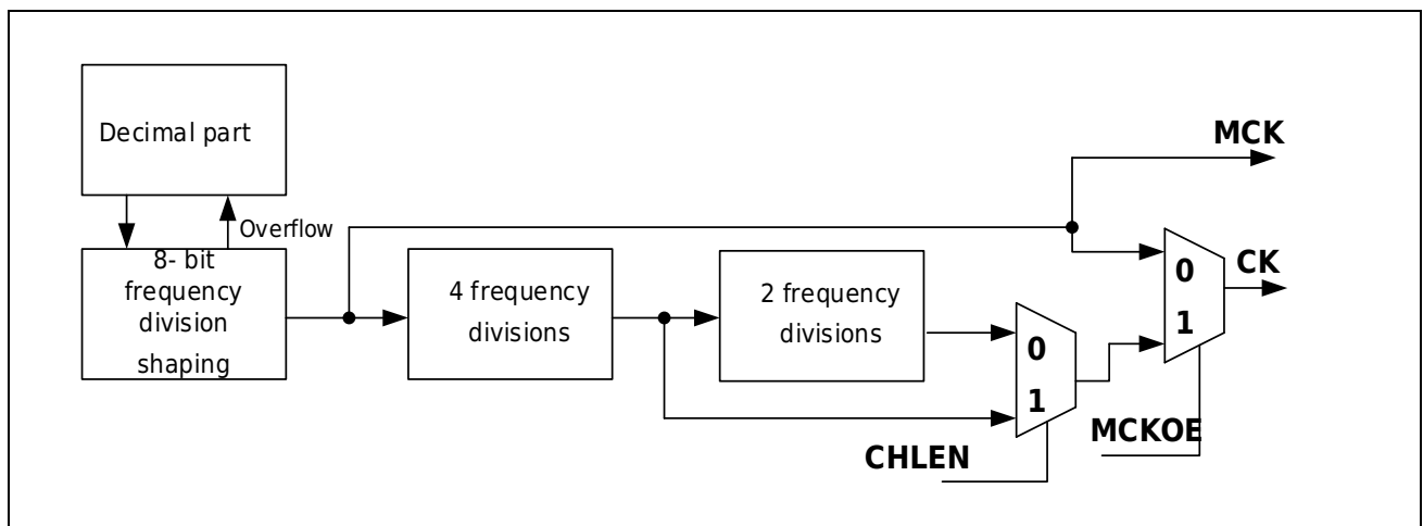
Figure 28-20 Clock Generation
