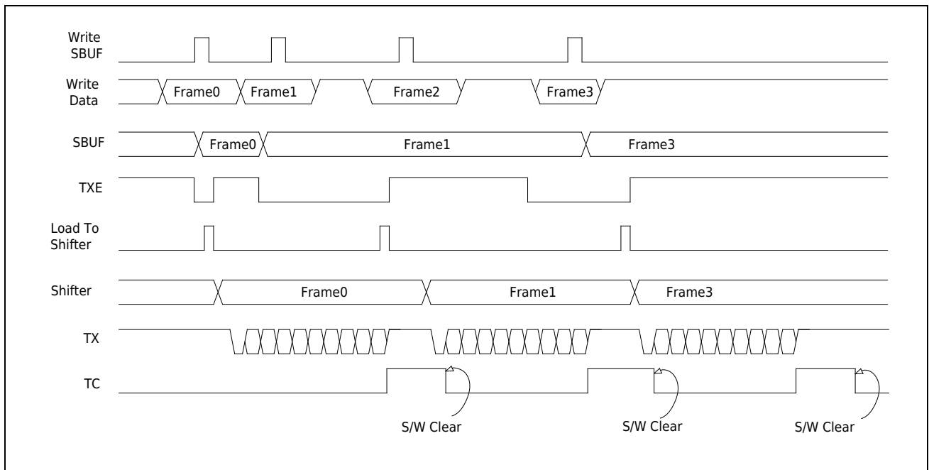
Figure 22-14 Send cache
