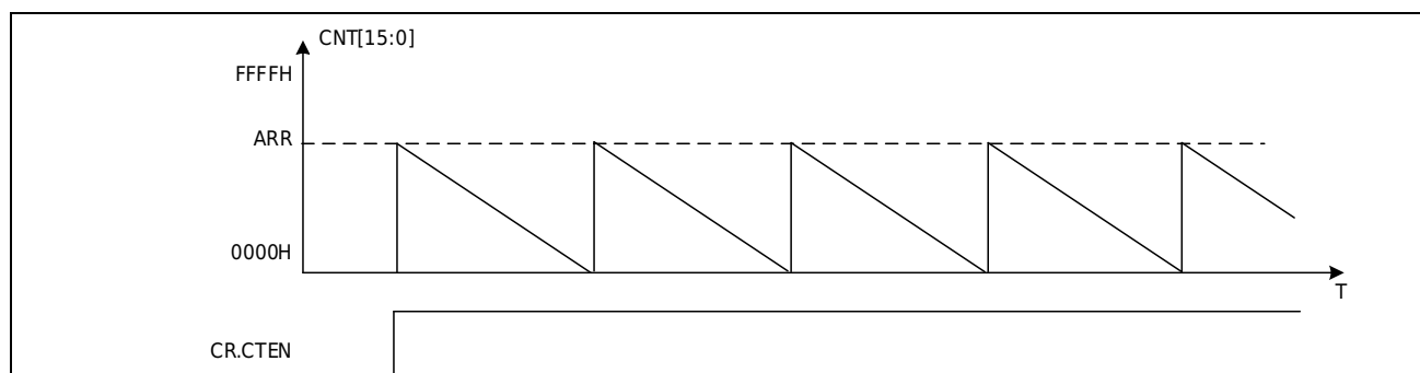
Figure 14-20 Edge-Aligned Timer Waveform (DIR = 1)
