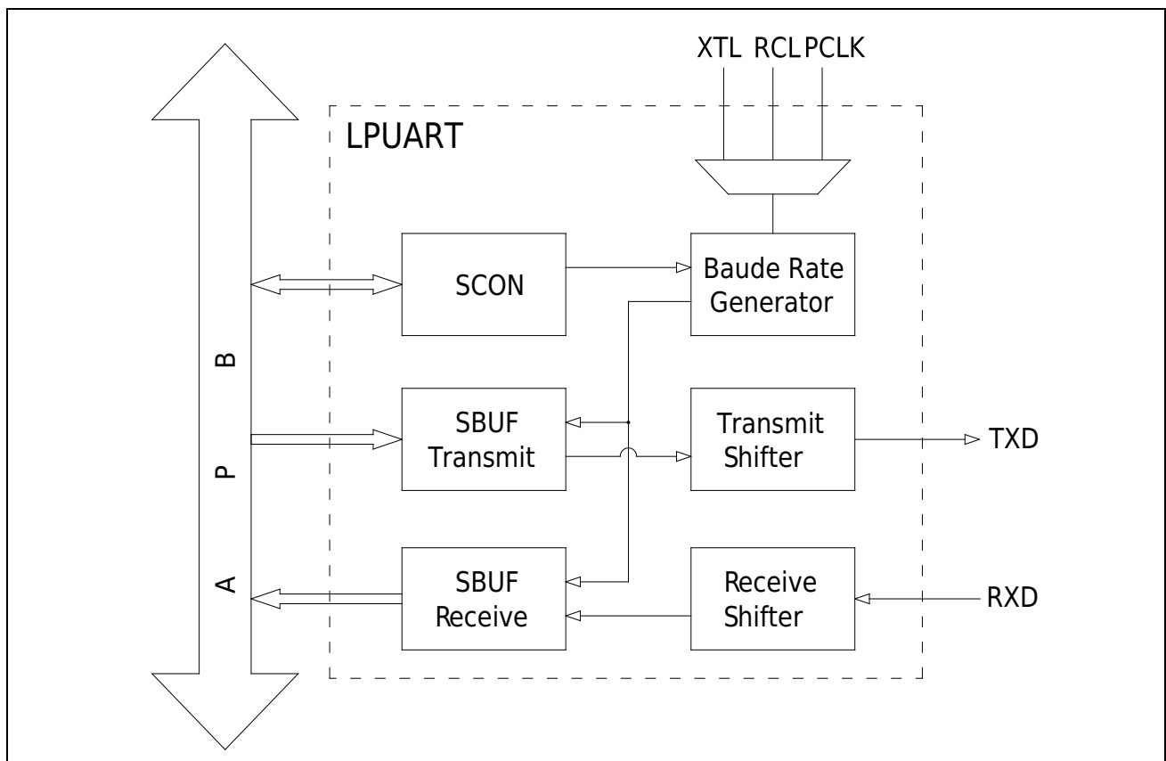
Figure 22-1 Block Diagram
