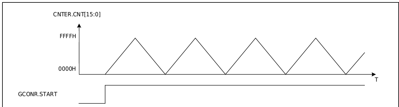
Figure 17-3 Triangle Waveform
