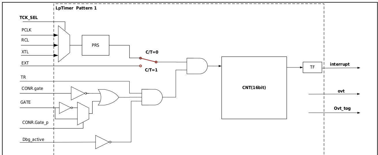
Figure 15-2 LPTimer Mode 1
