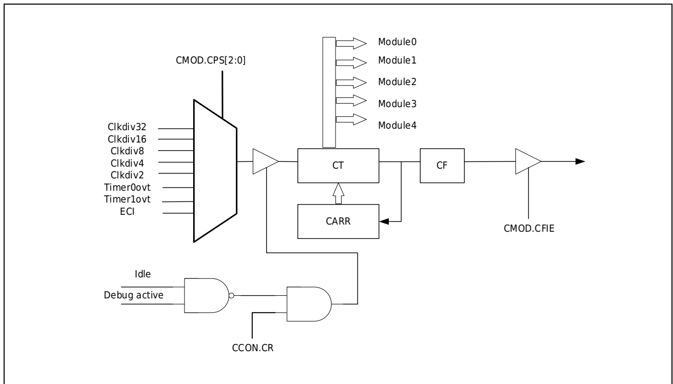
Figure 16-2 PCA Counter Block Diagram
