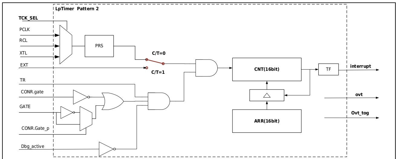
Figure 15-3 LPTimer Mode 2
