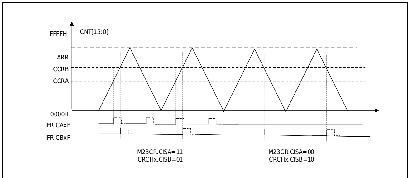
Figure 14-46 Interrupt diagram
