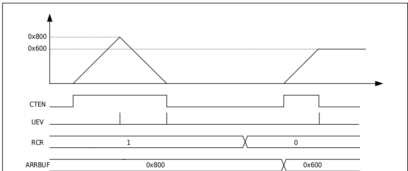
Figure 14-43 Single pulse counting in triangle wave mode
