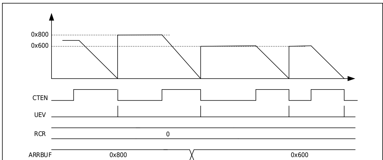
Figure 14-45 Counting single pulse mode under sawtooth waveform
