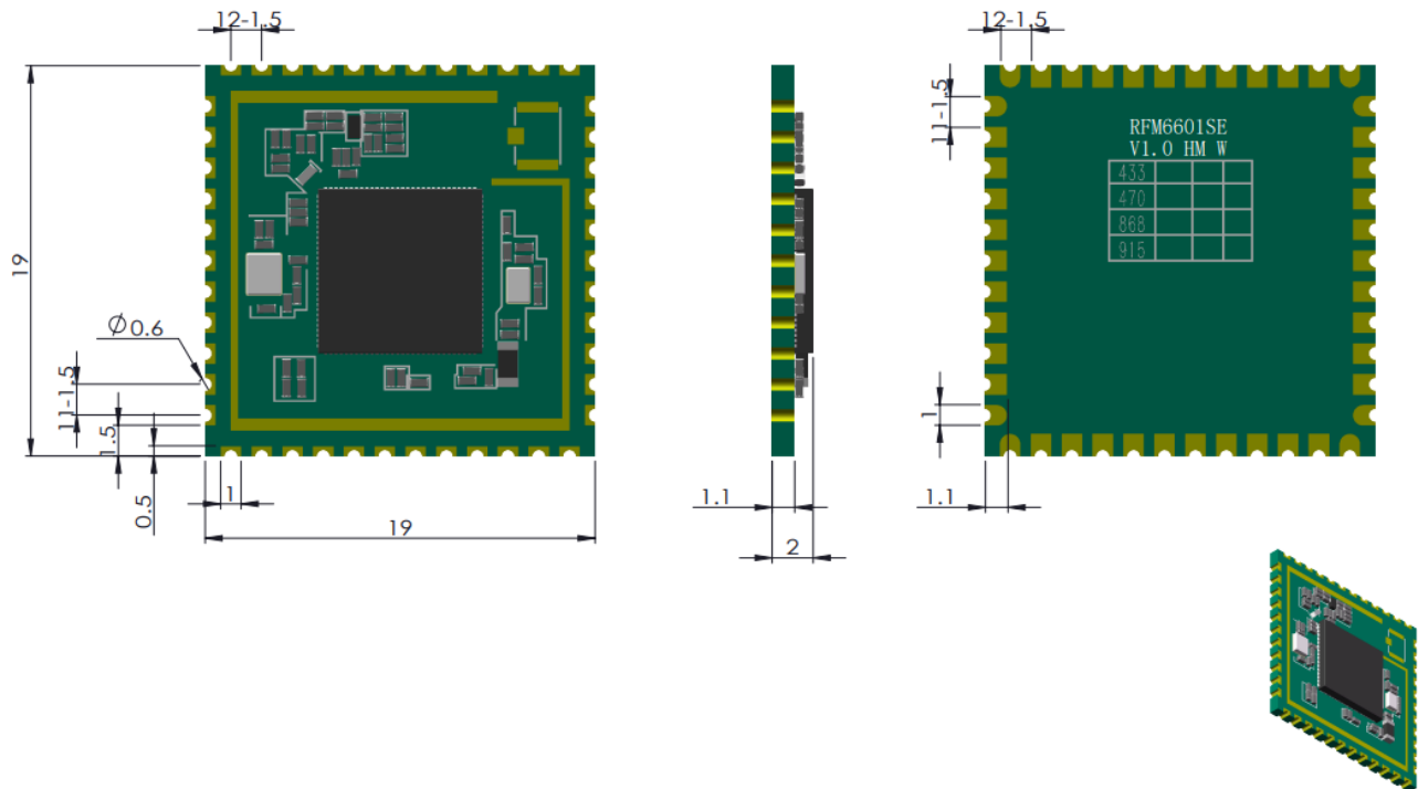
Figure 3. Dimension (unit: mm)
