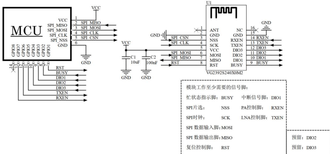
Figure 5- 2 Programming development hardware connection ( on-board PCB antenna )
