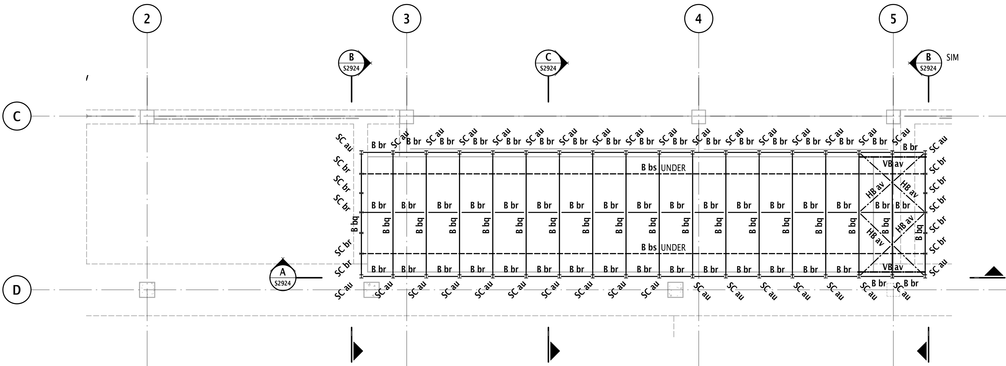
L13 ATRIUM ROOF STEEL FRAMING PLAN SCALE 1 : 100
