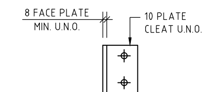
TYPICAL 10 PLATE T-CLEAT DETAIL U.N.O. 1:10
