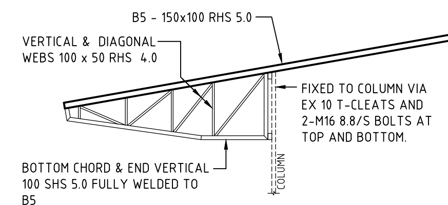
B5 FRAME-2 ELEVATION 1:50 FULLY WELDED FRAME
