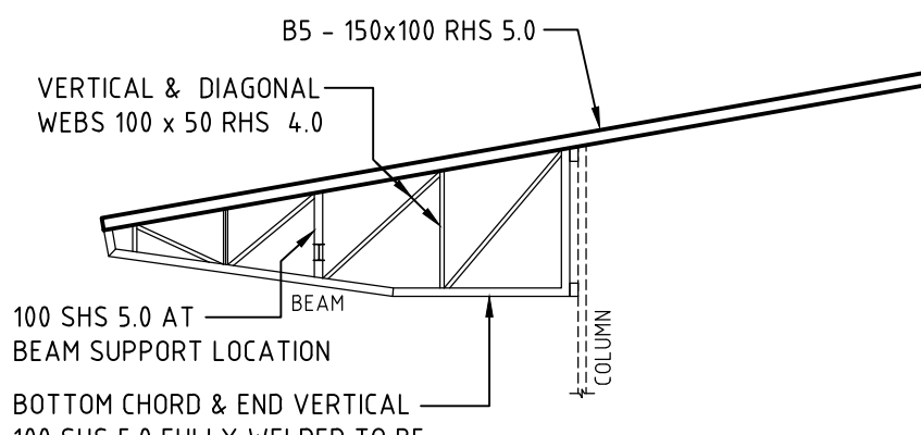
B5 FRAME-1 ELEVATION 1:50 FULLY WELDED FRAME
