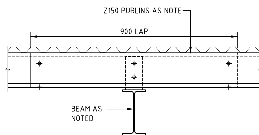
TYPICAL PURLIN LAP DETAIL 1:10
