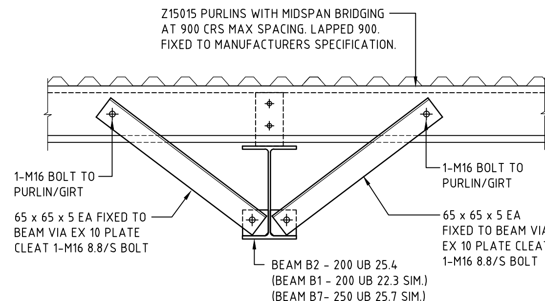
TYPICAL FLY BRACE DETAIL (fb) 1:10 PURLIN LAP FIXING OMITTED FOR CLARITY
