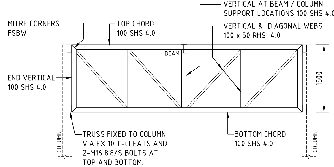
TYPICAL T1 TRUSS ELEVATION 1:50 FULLY WELDED FRAME
