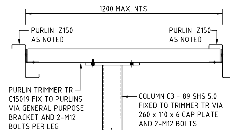
TYPICAL COLUMN TO PURLIN TRIMMER (TR) FIXING DETAIL 1:10
