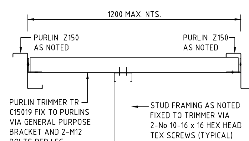
TYPICAL STUD TOP PLATE TO PURLIN TRIMMER (TR) FIXING DETAIL 1:10
