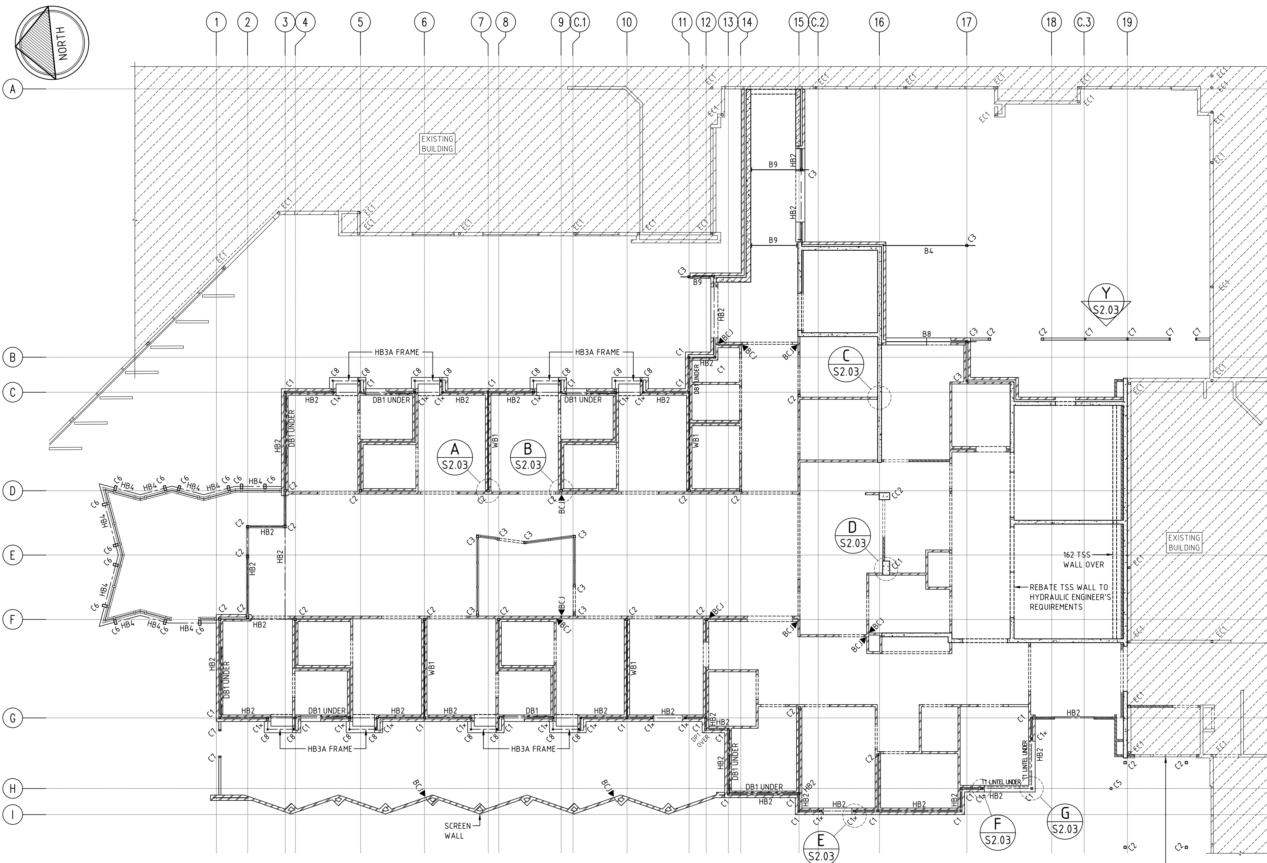
COLUMN AND WALL LAYOUT PLAN 1:100
