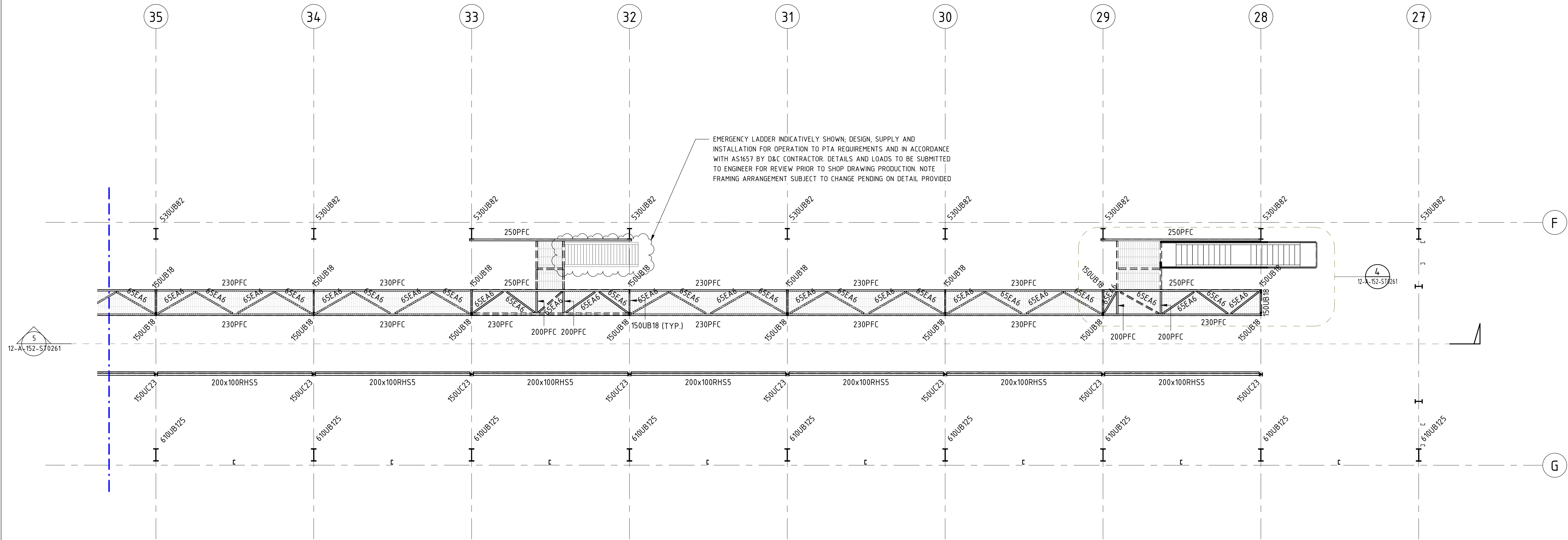
MEZZANINE STEELWORK PLAN (ZONE 3) 1 : 100
