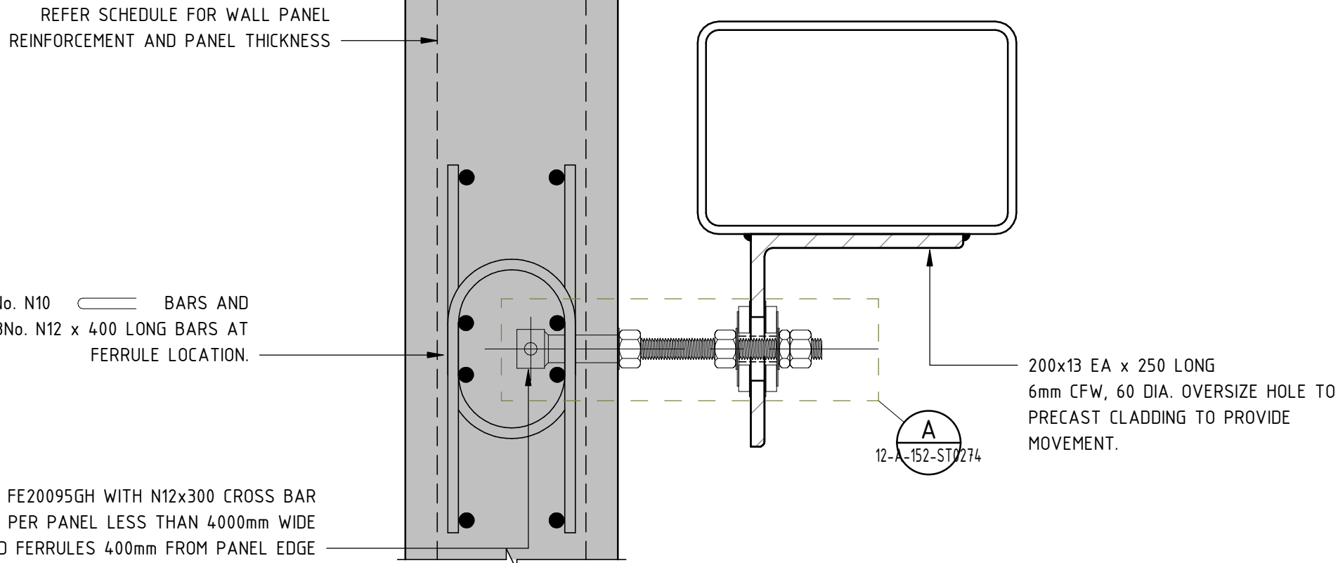
CONNECTION TYPE PC-CN02
