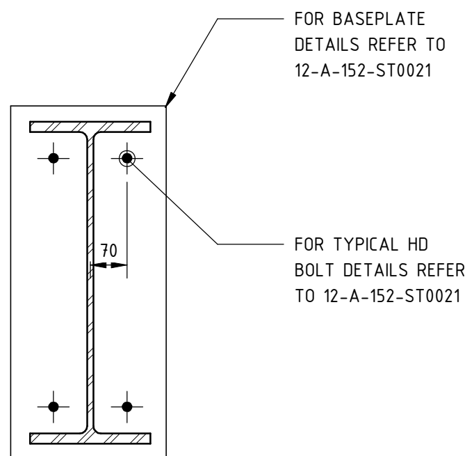
TYPICAL BASEPLATE DETAIL 1 : 10
