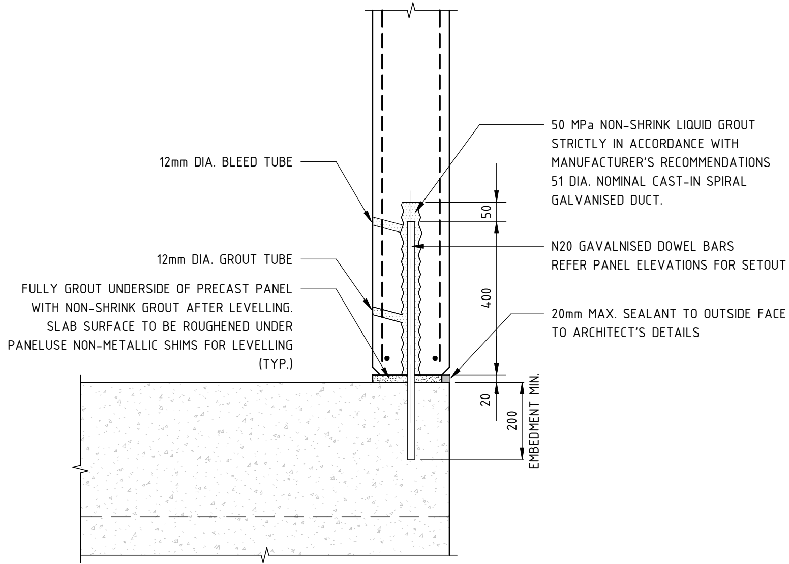
CONNECTION TYPE PC-CN01
