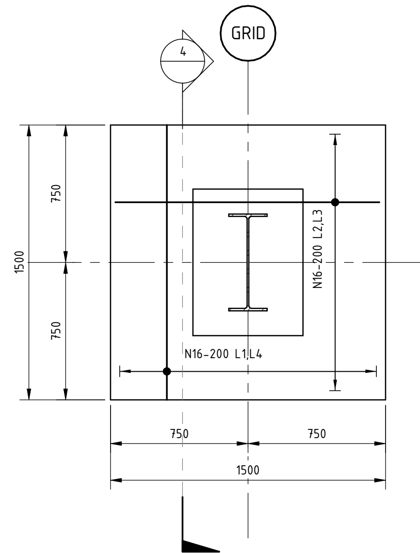
PF3 PAD FOOTING PLAN
