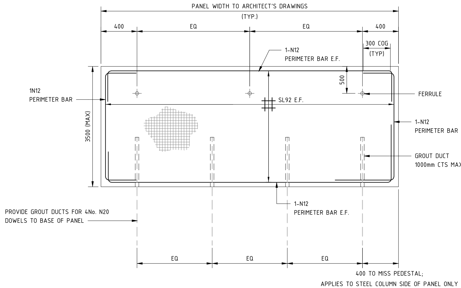
TYPICAL PANEL TYPE "PC01"
