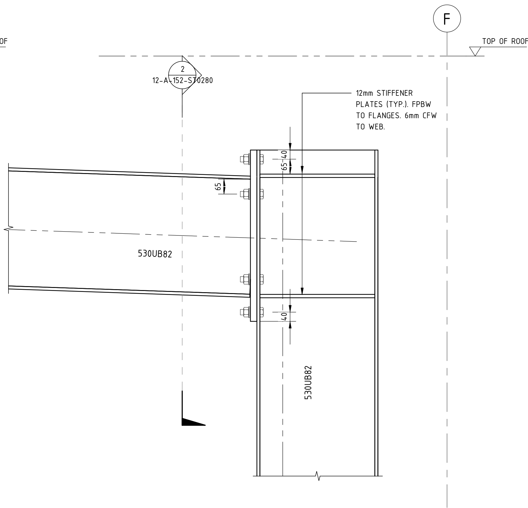
DETAIL 6 1 : 10 12-A-152-ST0258
