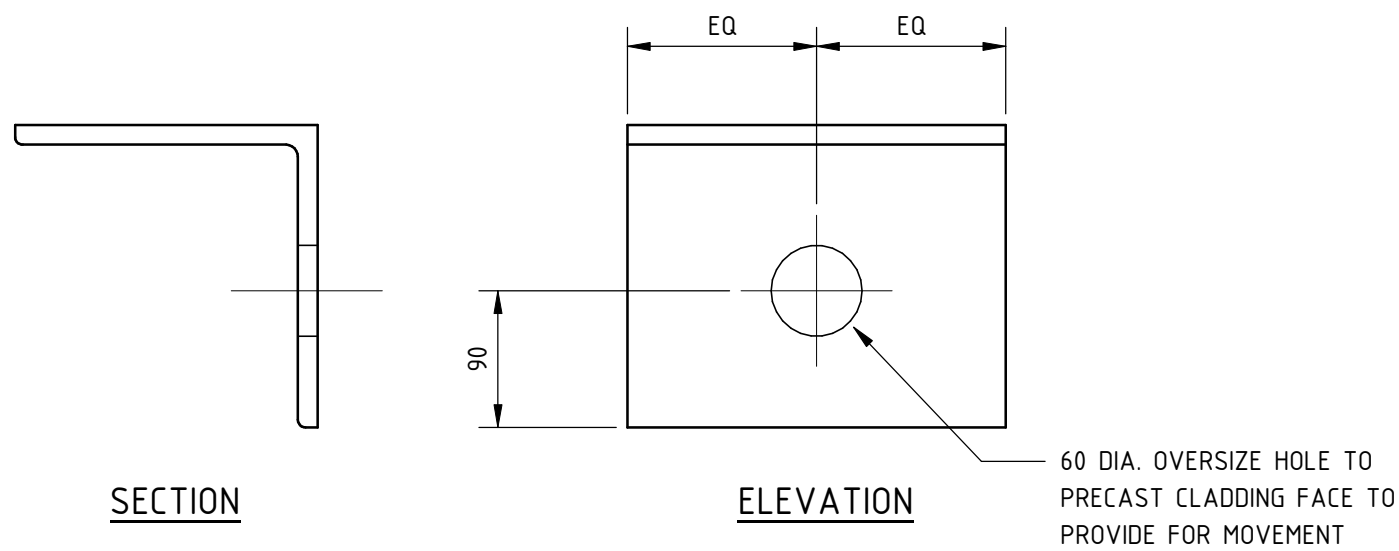
DETAIL B: TYPICAL ANGLE BRACKET
