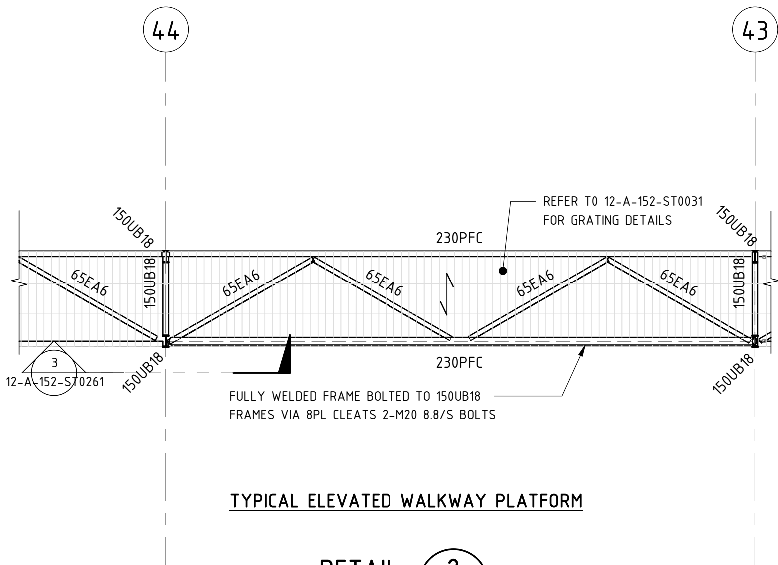
DETAIL 2 1 : 50 12-A-152-ST0221
