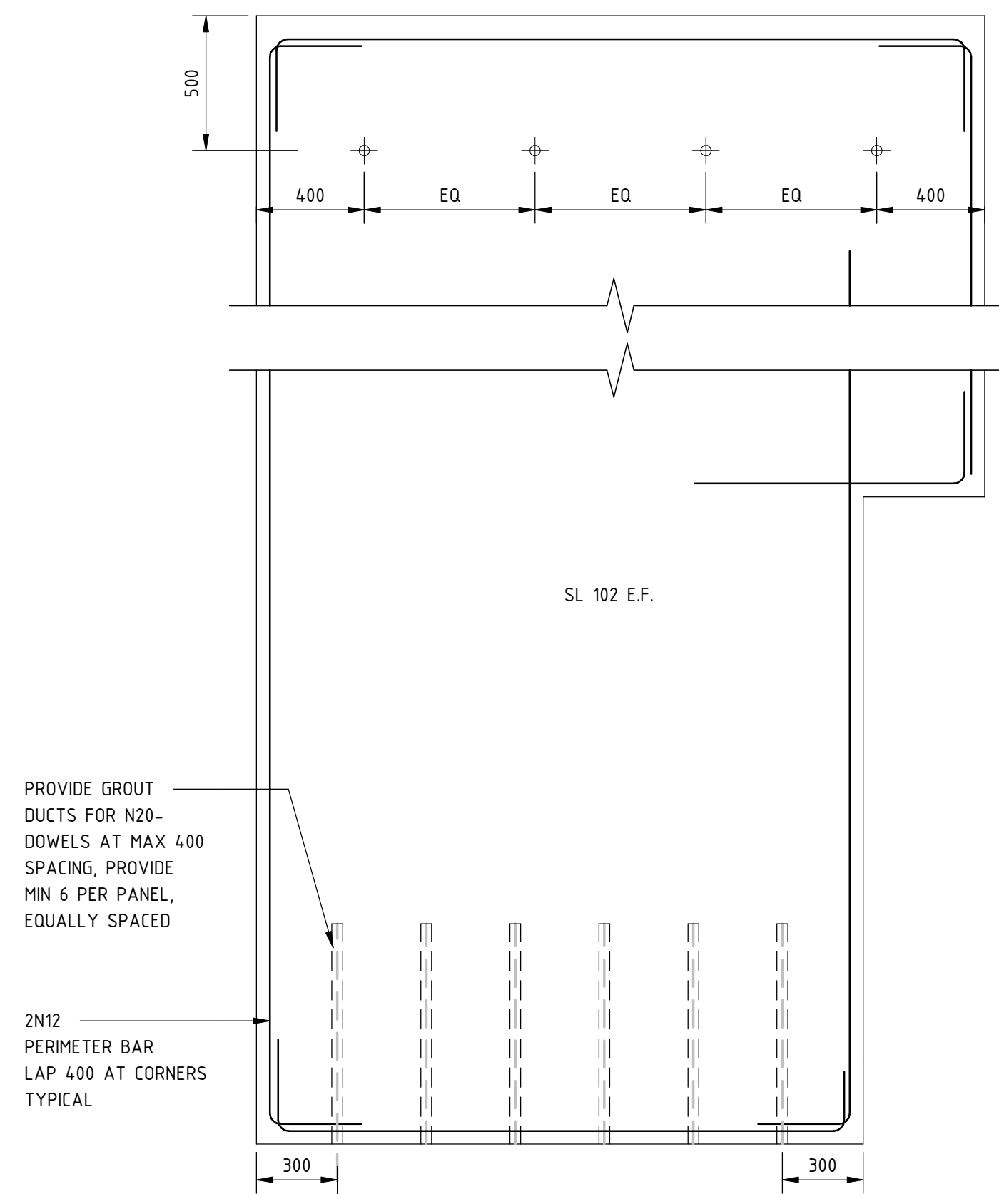
TYPICAL PANEL TYPE "PC-03"
