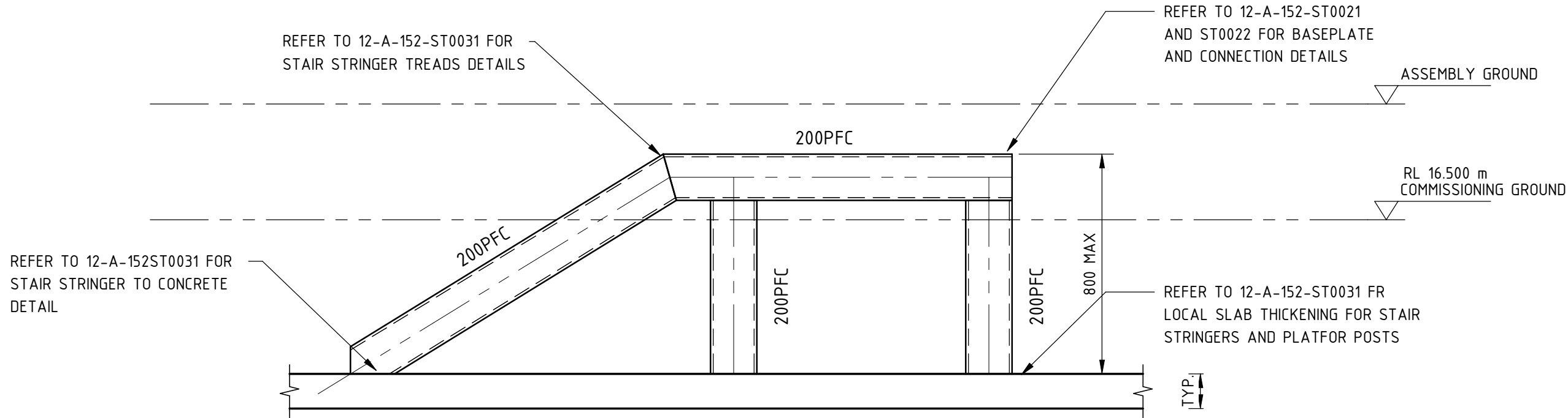
TYPICAL LOW LEVEL STAIR PLATFORM ELEVATION 1 : 20
