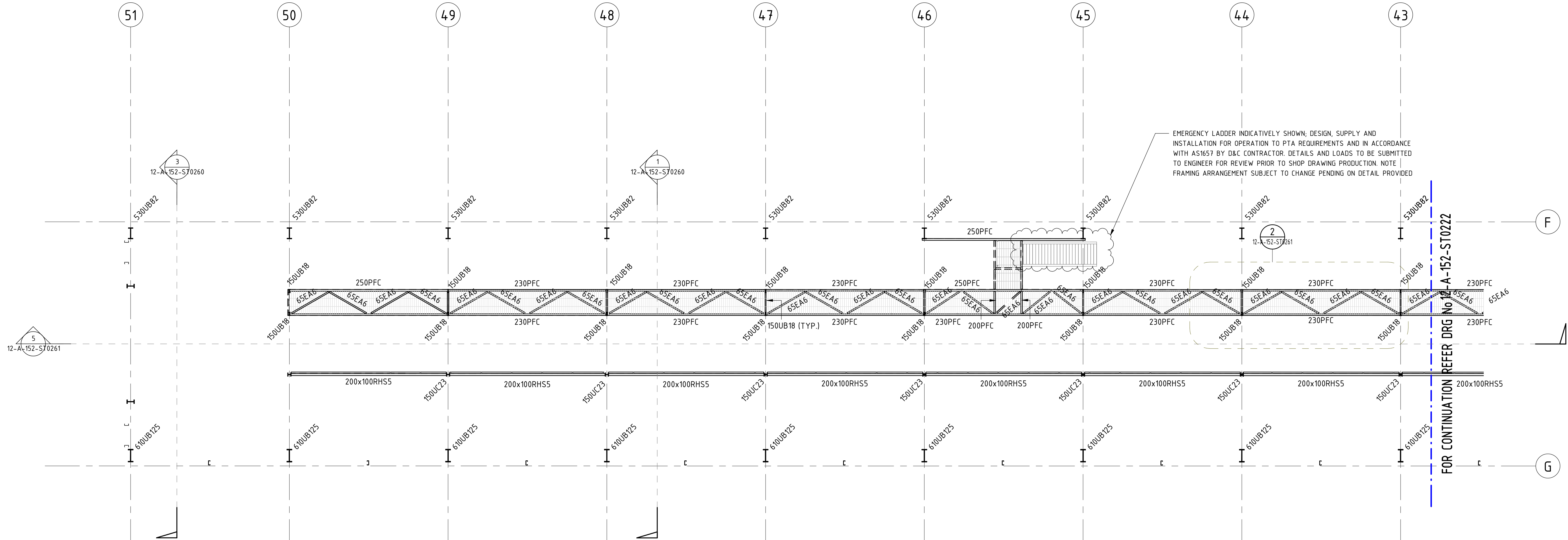
MEZZANINE STEELWORK PLAN (ZONE 1) 1 : 100
