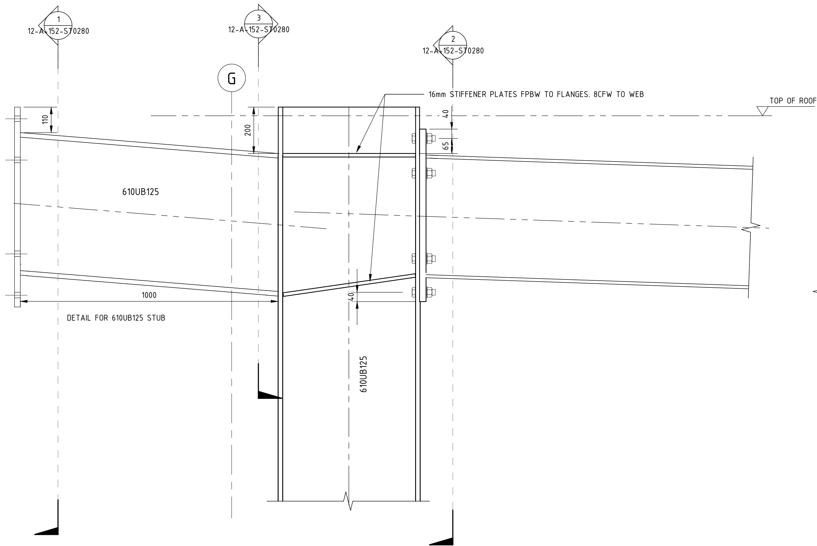
DETAIL 5 1 : 10 12-A-152-ST0258
