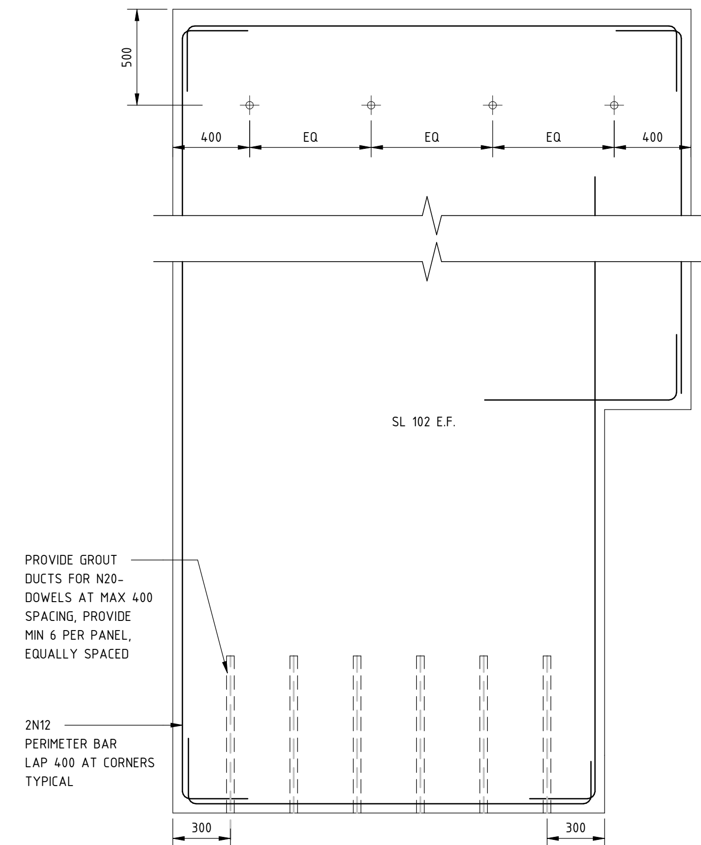
PRECAST PANEL: 200 STRUCTURAL THICKNESS
