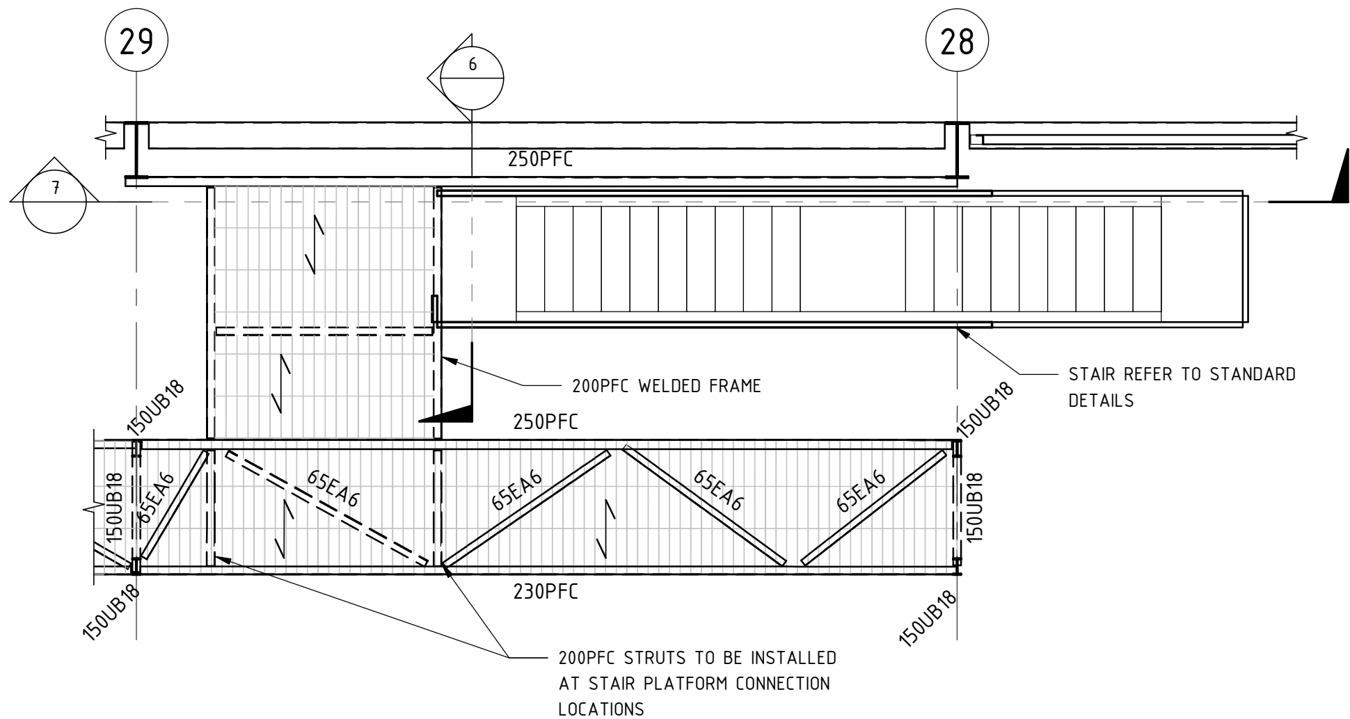
DETAIL 4 1 : 50 12-A-152-ST0223
