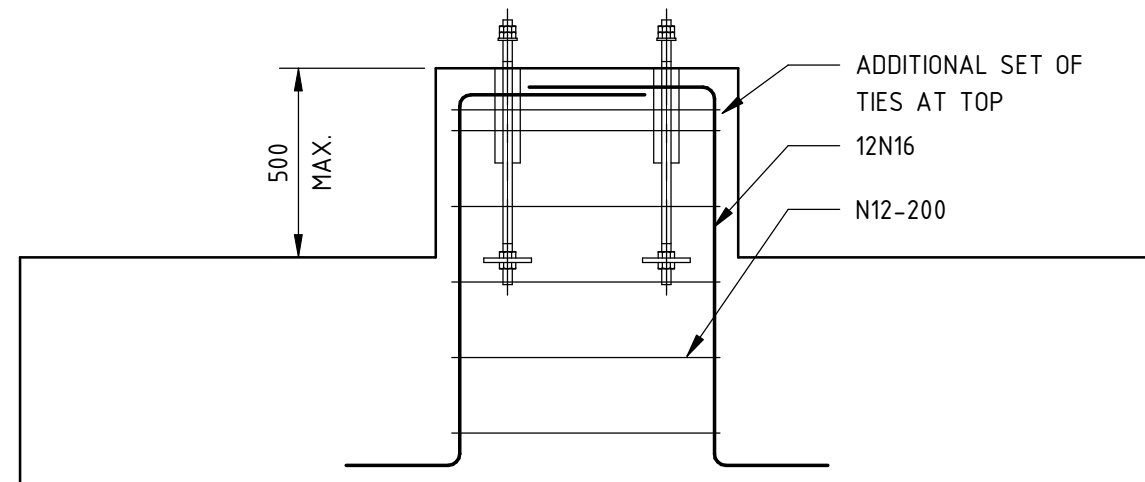
SECTION THROUGH P2
