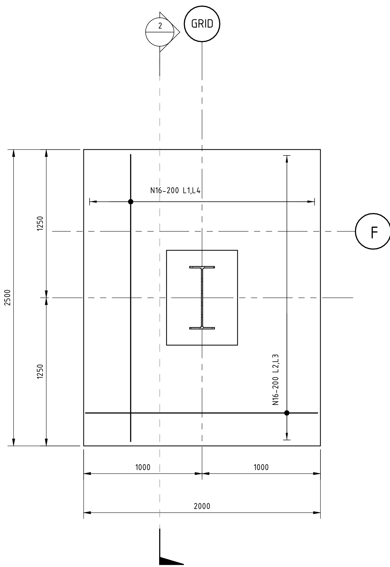
PF1 PAD FOOTING PLAN
