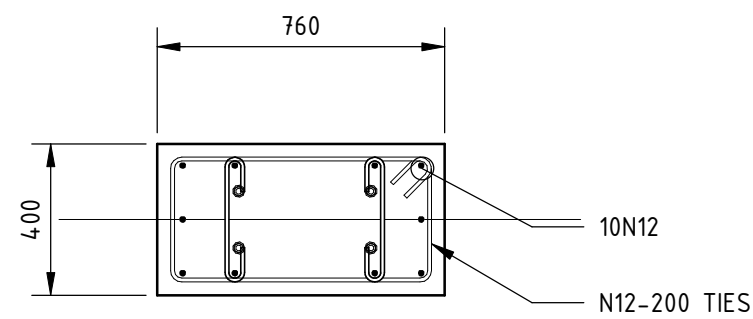
TYPICAL SECTION THROUGH P2
