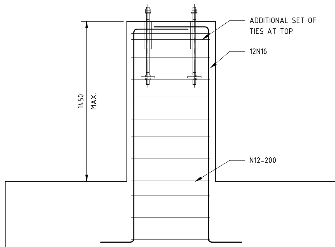
SECTION THROUGH P1
