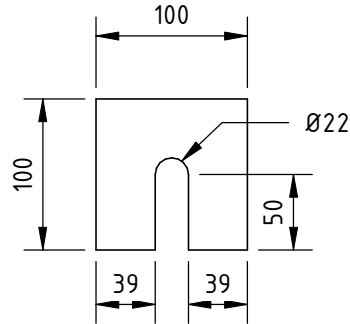
PACKER PLATE DETAIL
