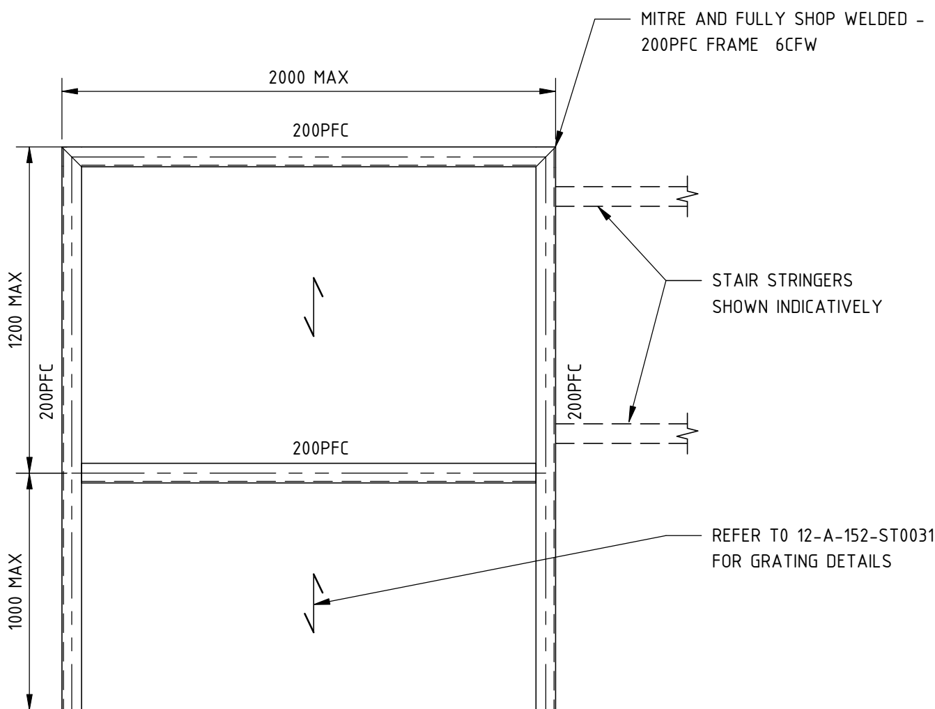
200PFC WELDED FRAME STAIR LANDING PLATFORM PLAN 1 : 20
