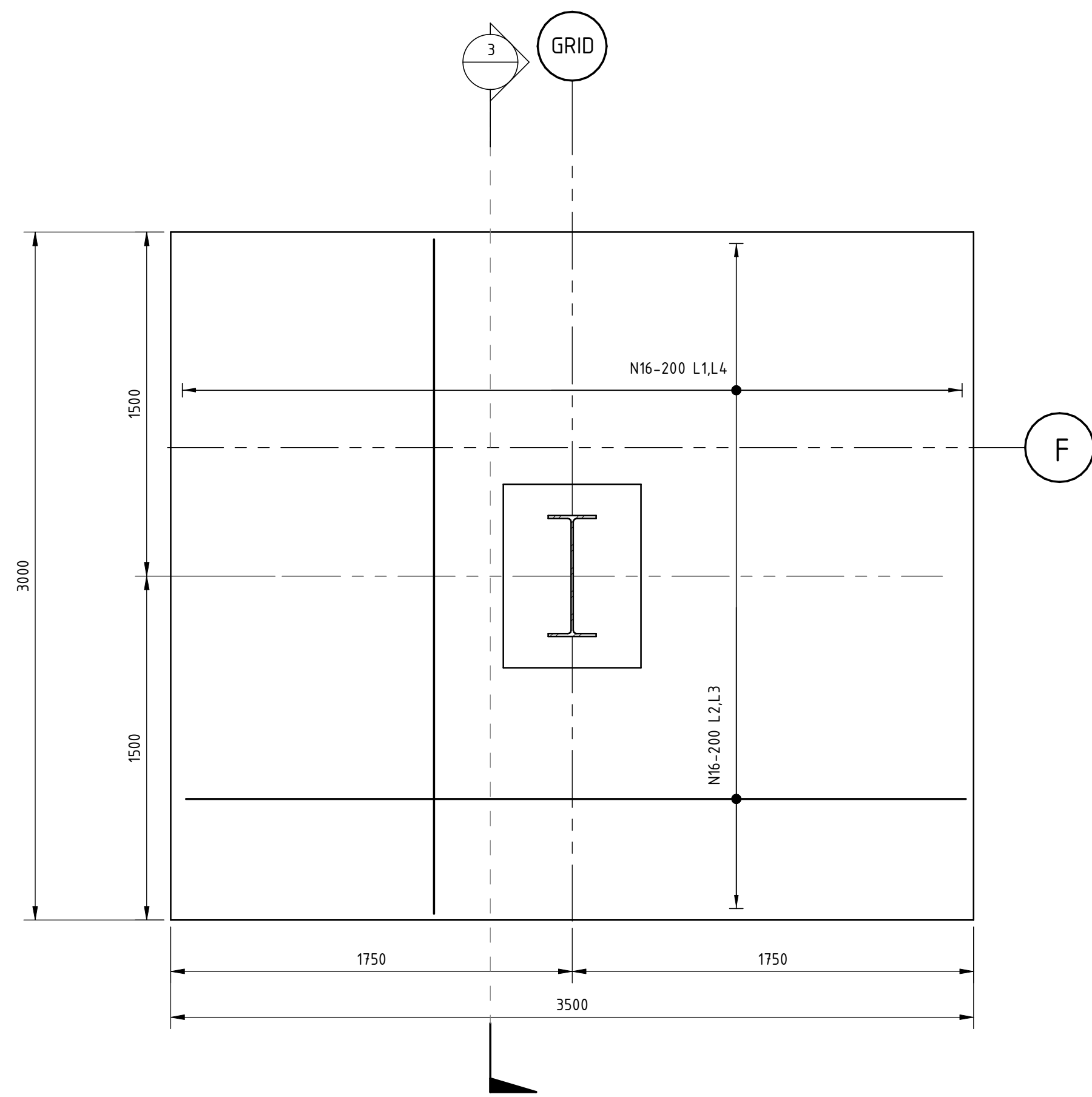
PF2 PAD FOOTING PLAN
