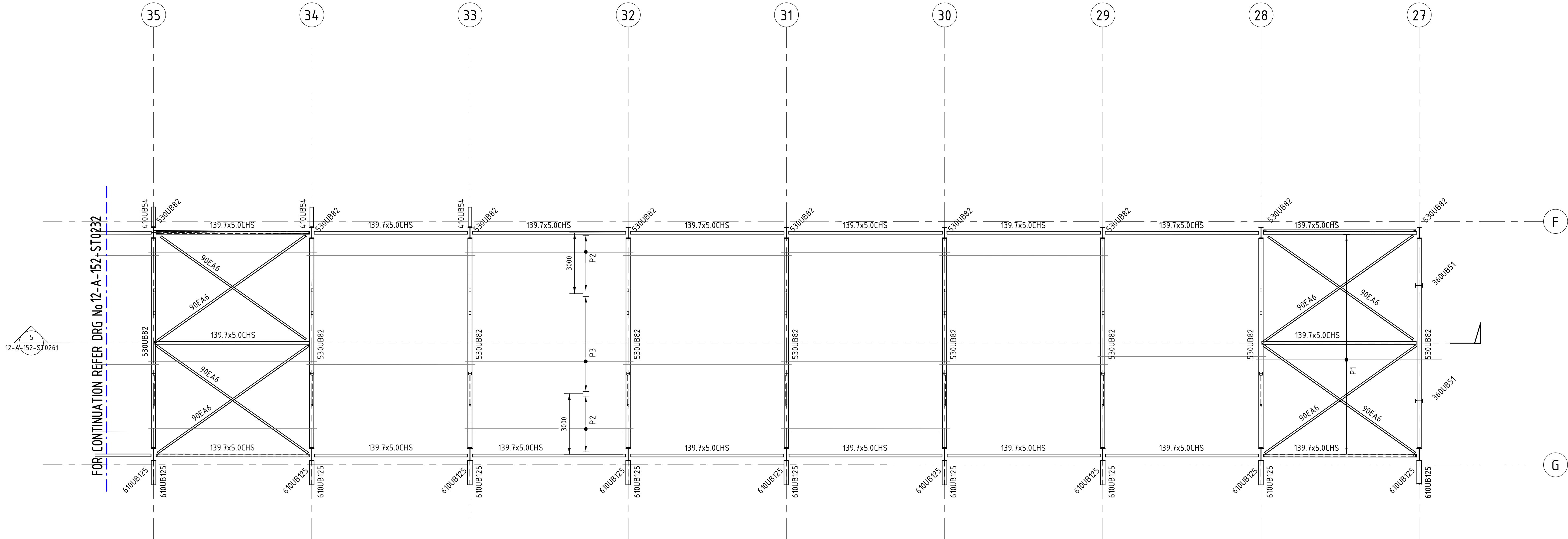
OVERALL ROOF PLAN (ZONE 3)
