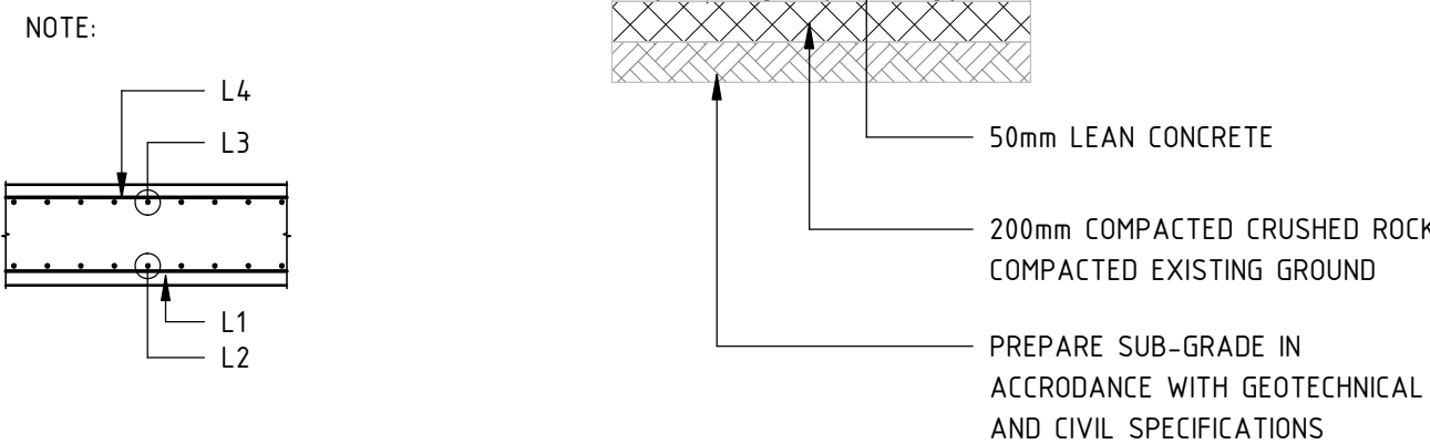
REINFORCEMENT KEY TYPICAL COMPACTION DETAIL
