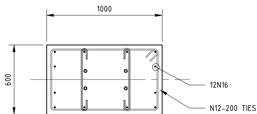
TYPICAL SECTION THROUGH P1
