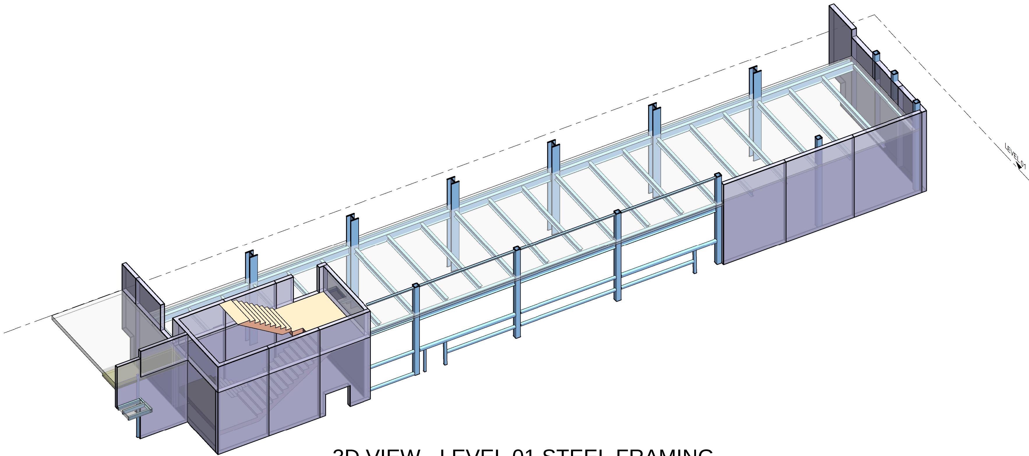
3D VIEW - LEVEL 01 STEEL FRAMING
