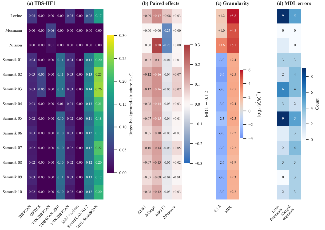
Fig. 3. Biological results without pooling datasets. (a) Post-hoc target–background–structure harmonic F1; all-assigned k NN+Leiden scores zero. (b) Paired changes in TBS and its target, background, and pairwise constituents. (c) Predicted-to-annotated cluster-count ratio. (d) MDL target fragmentation and merging counts.
