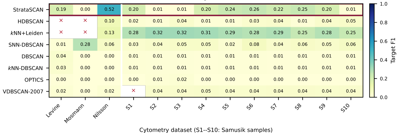
One-to-one macro target F1; absolute values
