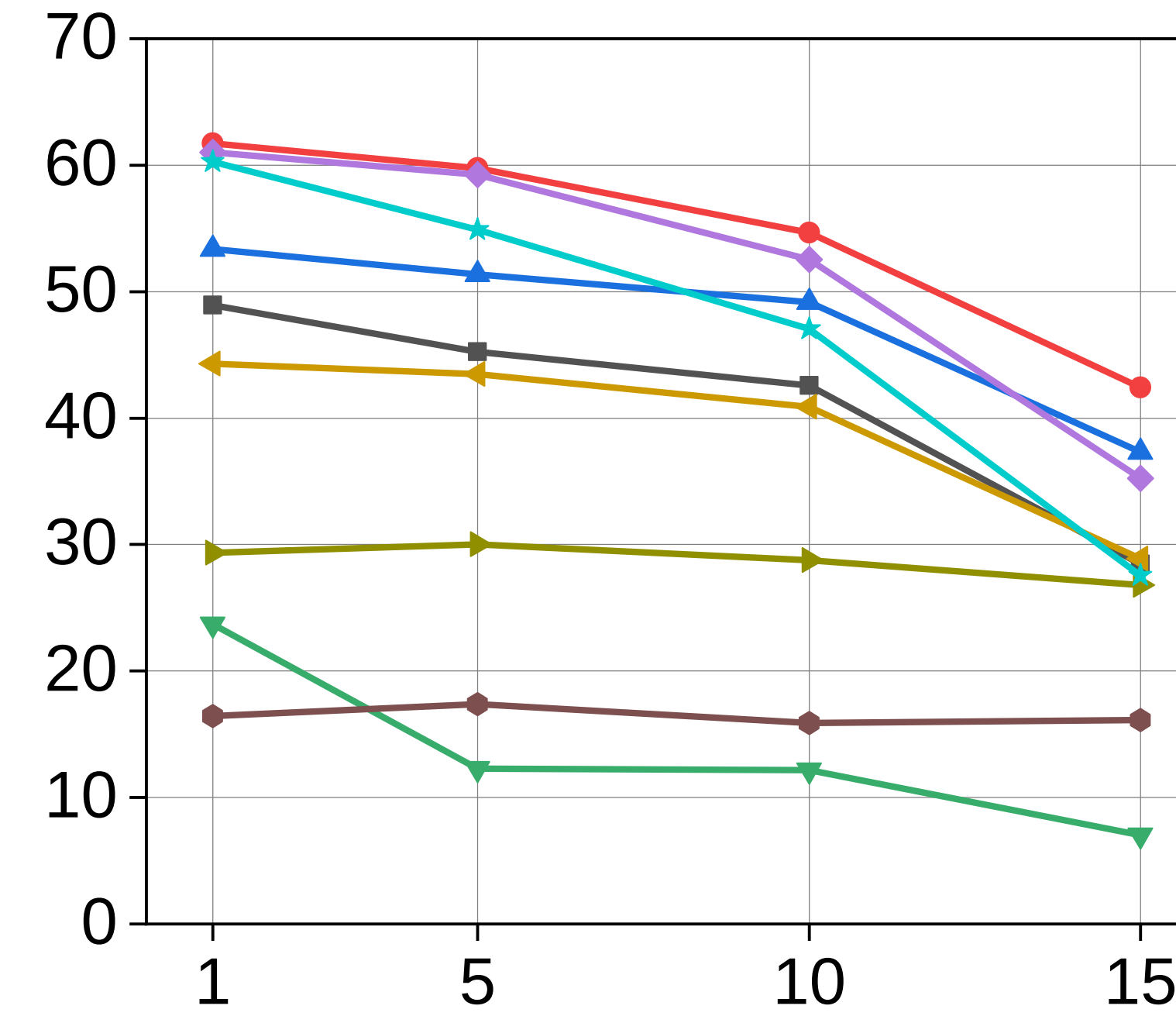
(c) IVDetect
