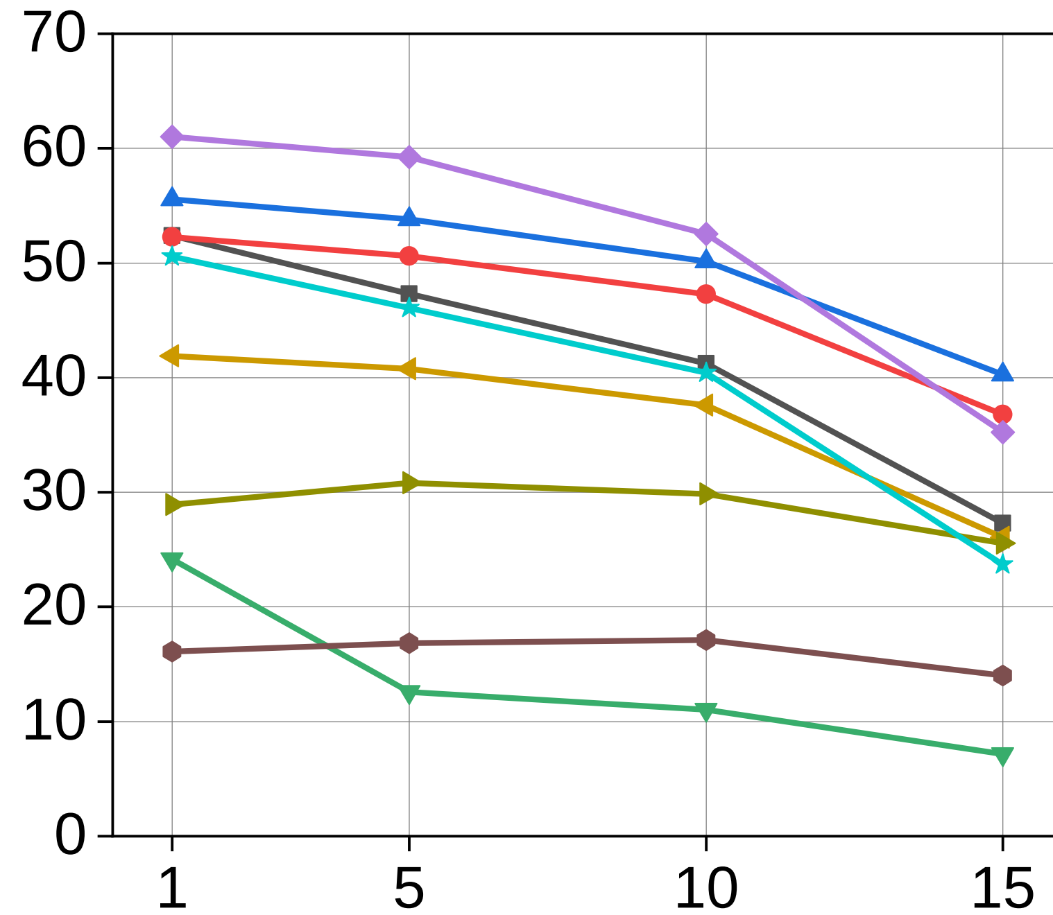
(a) Deepwukong
