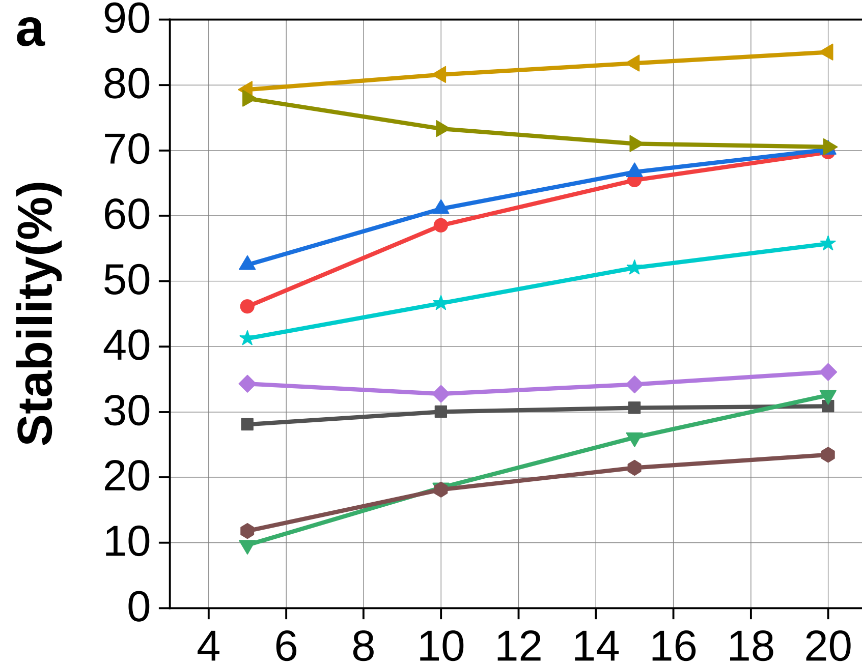
(a) Deepwukong
