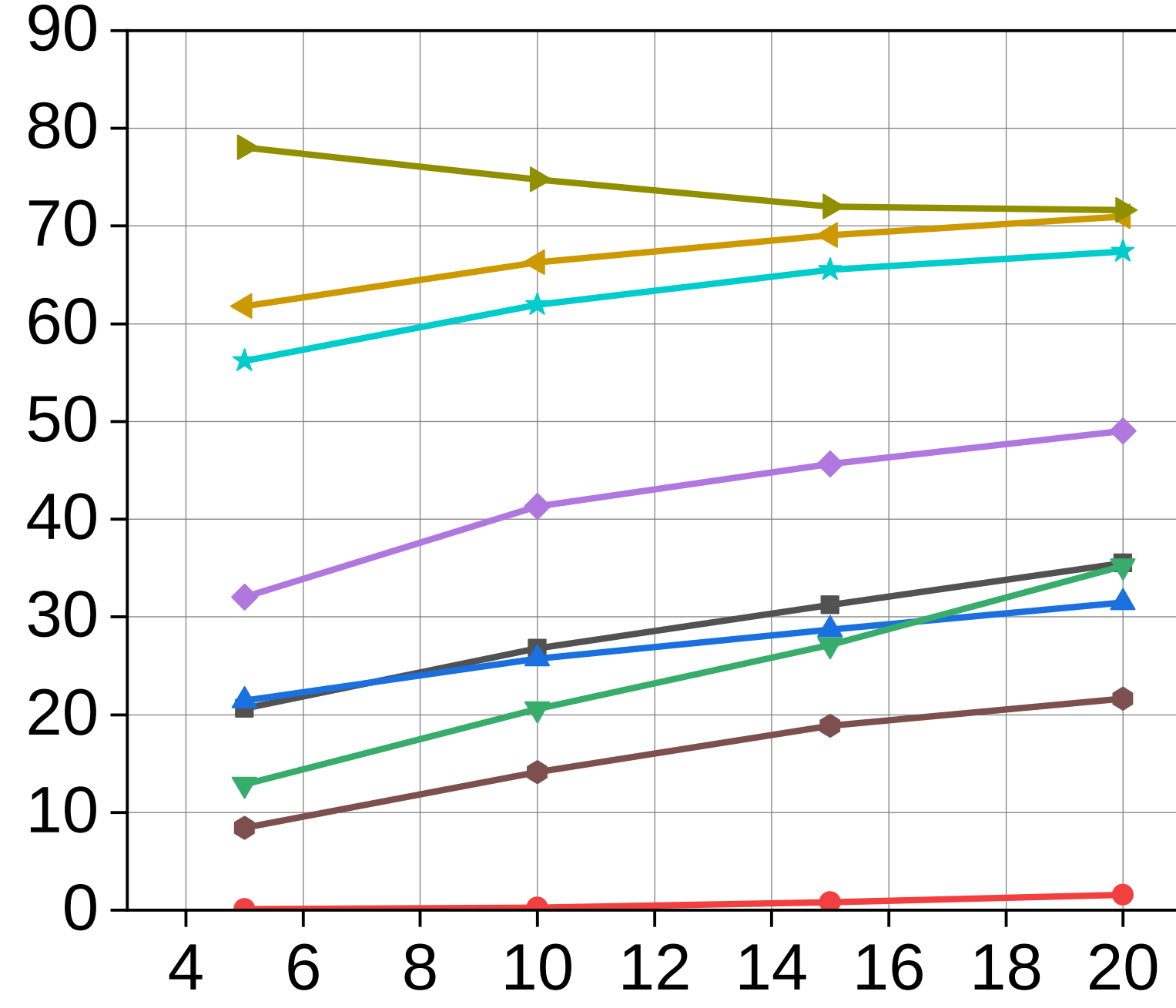
(c) IVDetect
