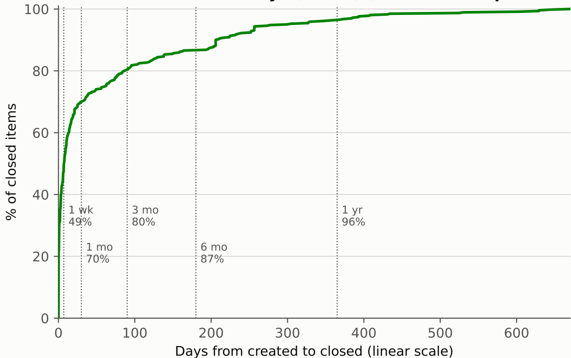
B % closed within N days (linear) (excl. svc-completeness)
