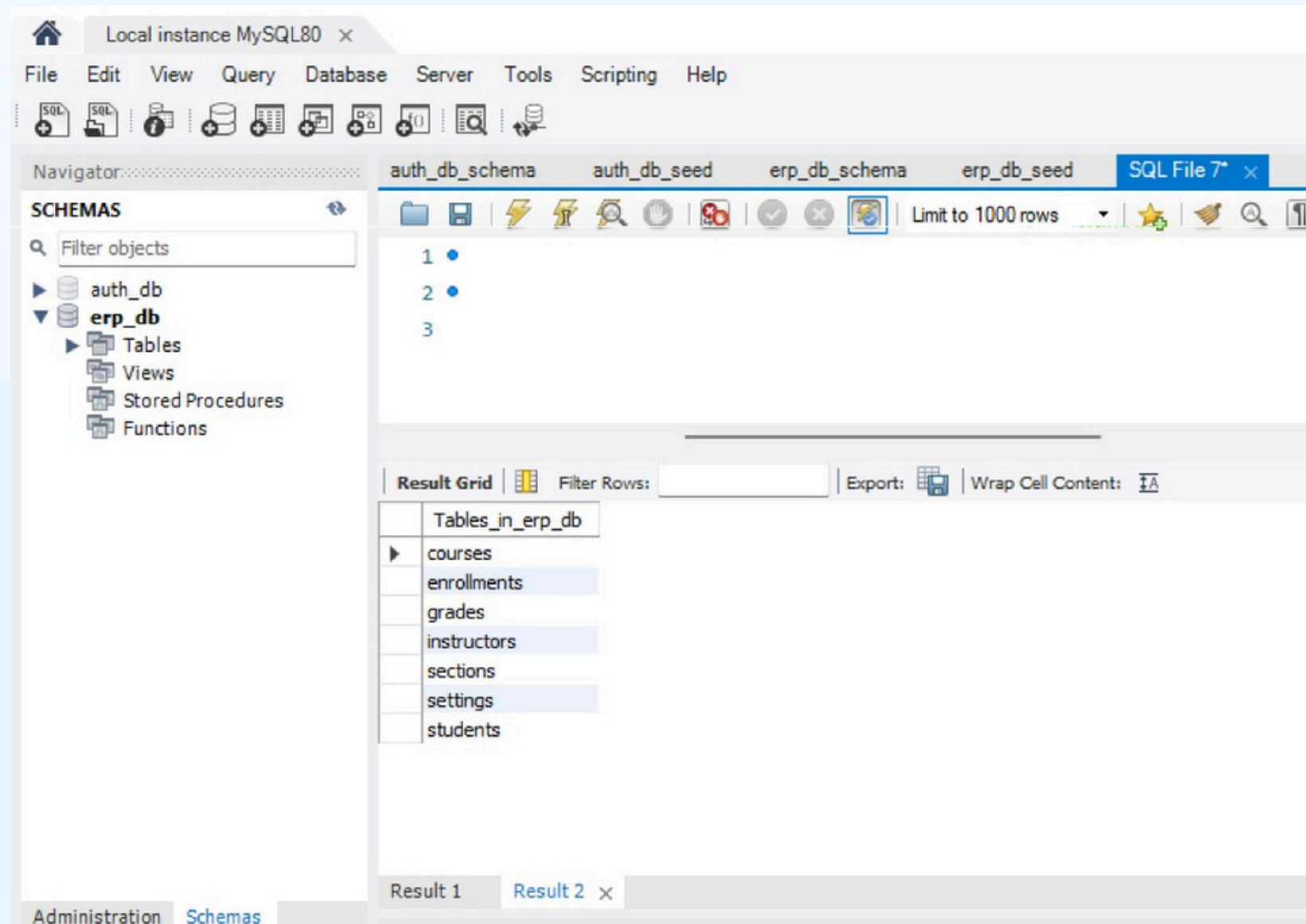
Erp DB
