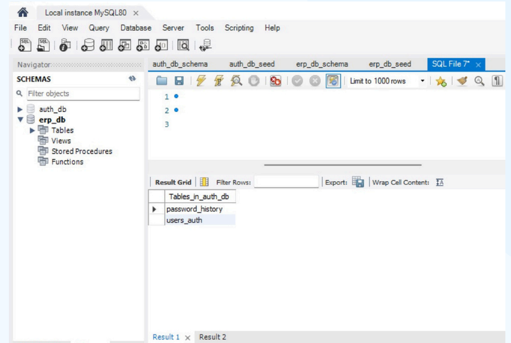
Auth DB
