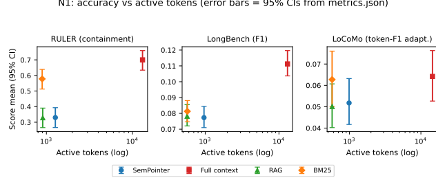
Fig. 2. Lead result: measured accuracy versus measured active tokens (Pareto plane), one panel per suite, with 95% CIs. SemPointer sits an order of magnitude left of full context on tokens at lower accuracy, and ties dense RAG at higher token cost. KV-compress pilot omitted (n=10).
