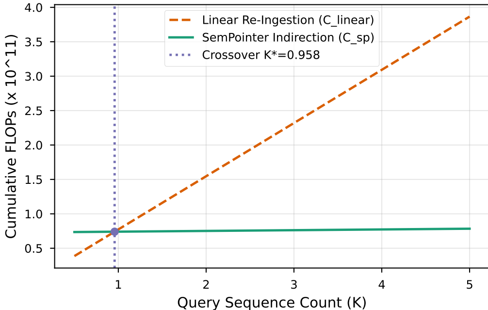
F1: Cumulative FLOPs Crossover (N=2, B=512, k=8)
