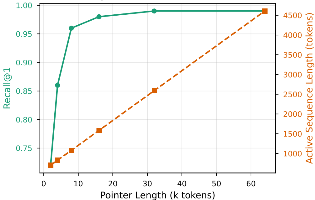
F6: Pointer Length (k) Pareto Tradeoff (N=64, B=512)
