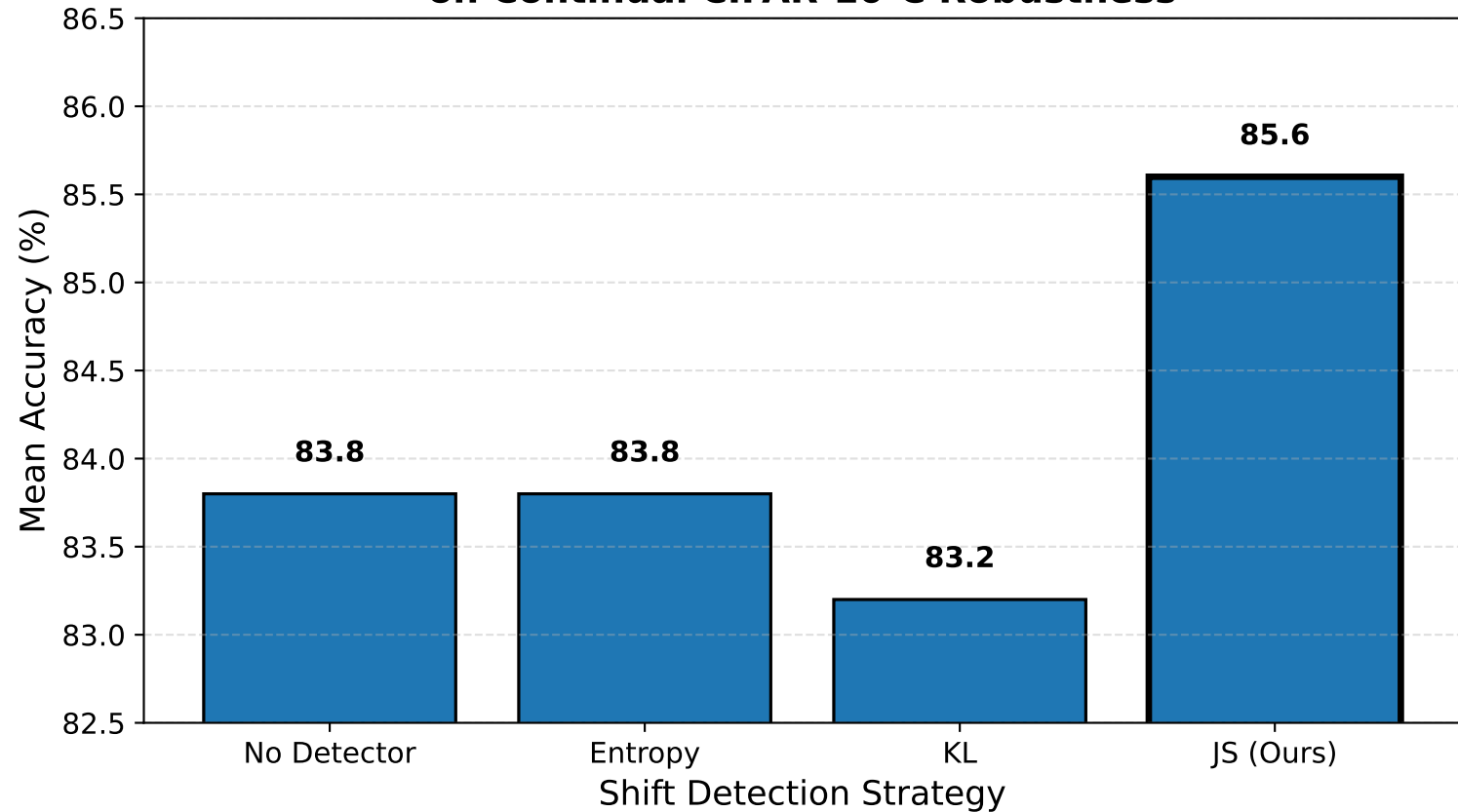
Effect of Shift Detection Strategy on Continual CIFAR-10-C Robustness
