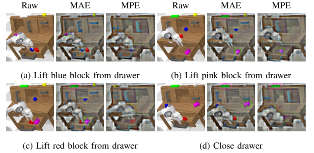
Fig. 3. Qualitative visualization of task-relevant reconstructions.
