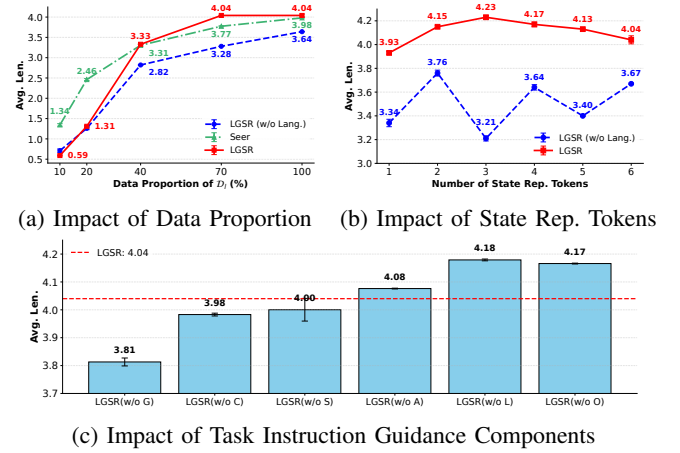
Fig. 2. Ablation Study. (a) Impact of data proportion on performance, where 100% corresponds to 17,870 language-annotated episodes. (b) Impact of the number of state representation (Rep.) tokens on performance. (c) Impact of different components in task instruction guidance on performance. G: Goal; C: Constraint; S: Spatial; A: Action; L: Logic; O: Other. The error bars denote standard error of the mean (SEM).
