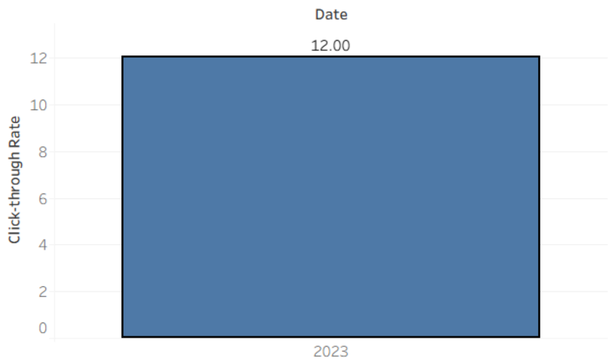
Click-through Rate.
