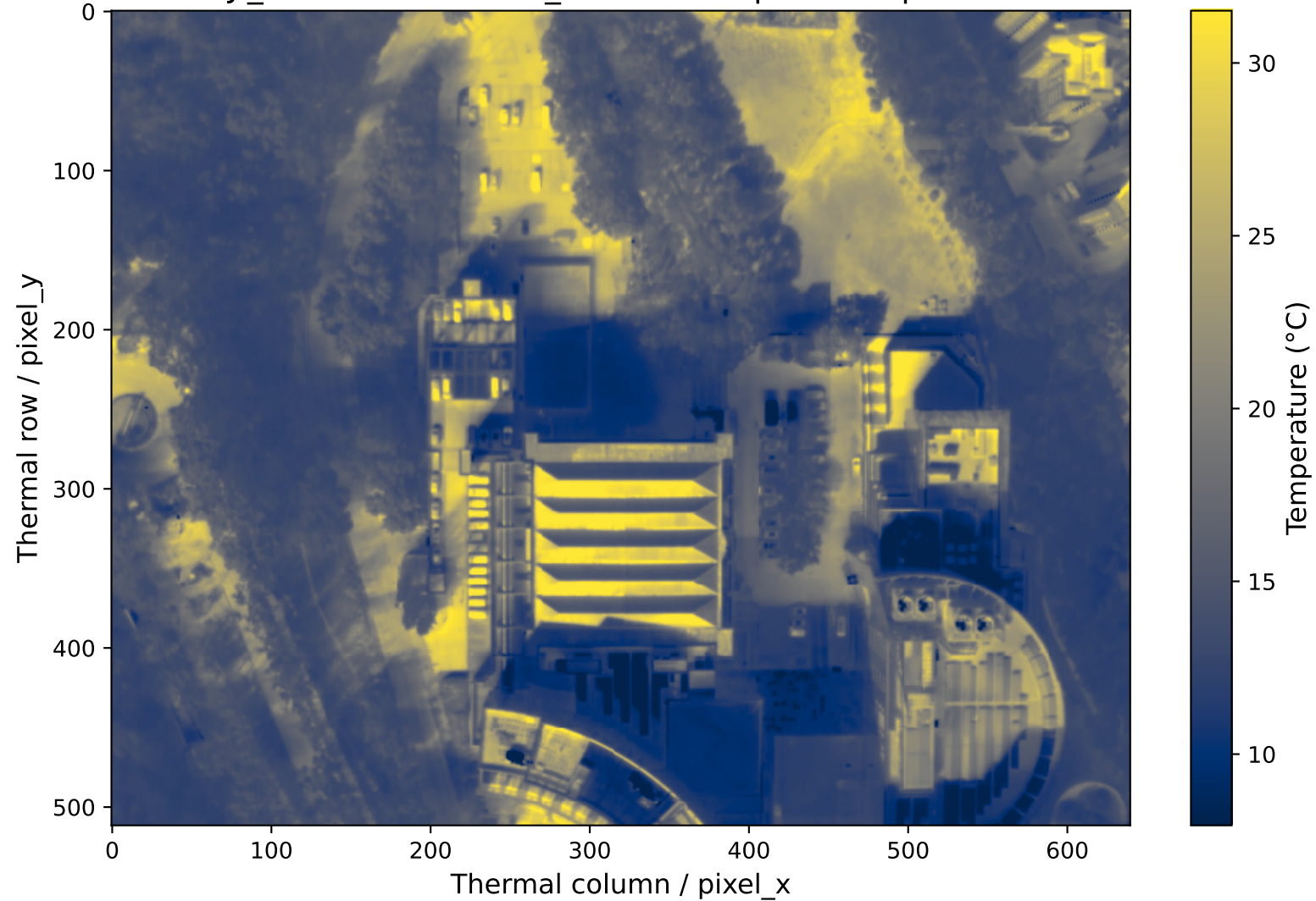
DJI_20260107143320_0007 — full-pixel temperature
