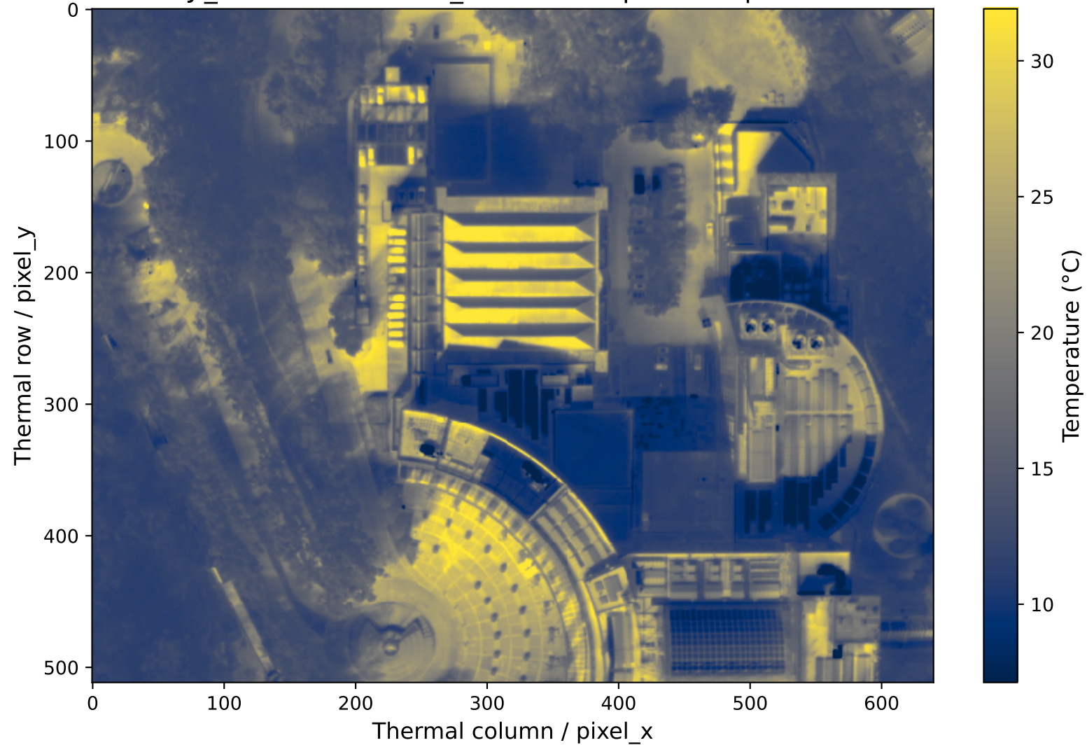
DJI_20260107143328_0008 — full-pixel temperature
