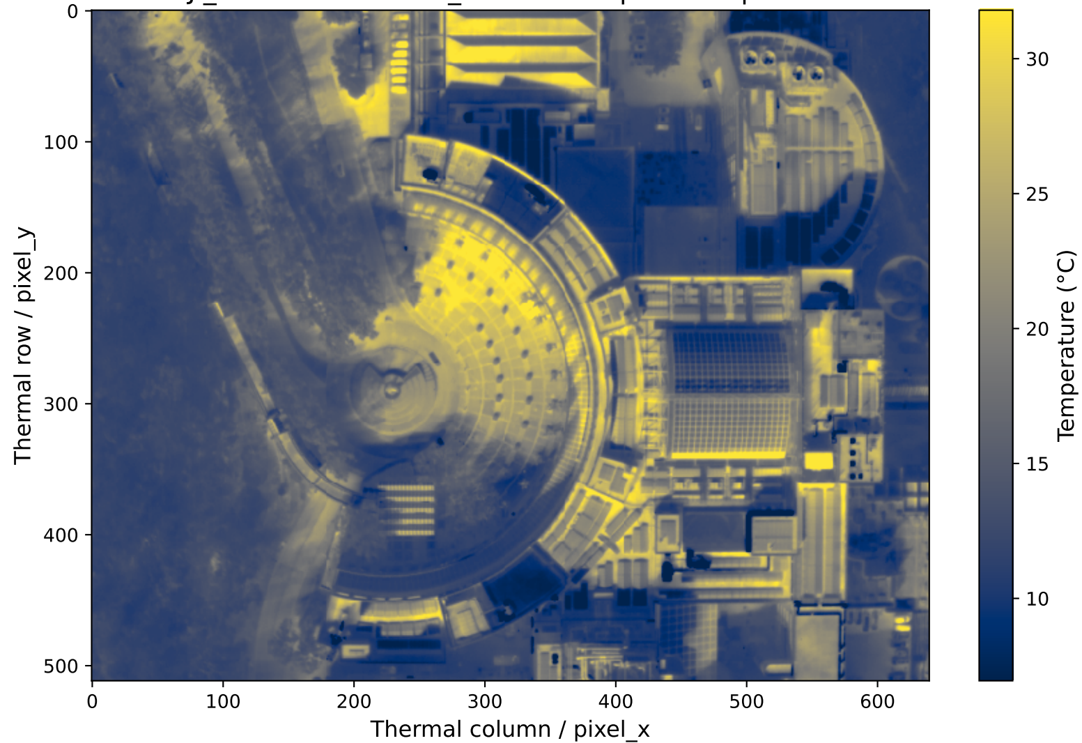
DJI_20260107143344_0009 — full-pixel temperature
