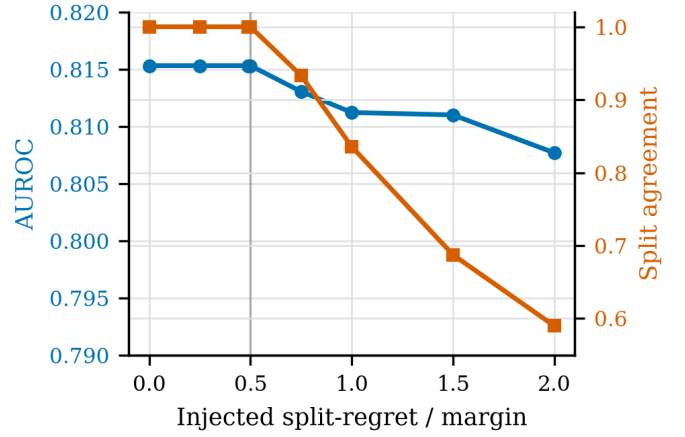
Fig. 6: Robustness pattern. Split agreement drops after dose 0.5; AUROC degrades mildly as calibrated split-gain noise exceeds the margin. The vertical line marks the dose 0.5 margin boundary.
