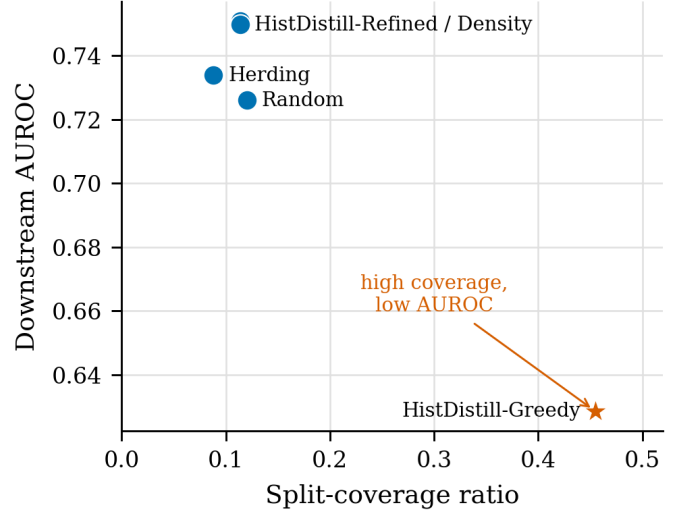
Fig. 4: Coverage versus downstream AUROC. HD-Greedy covers the most high-gain split thresholds, but the higher-AUROC methods occupy a different region of the coverage-AUROC plane.
