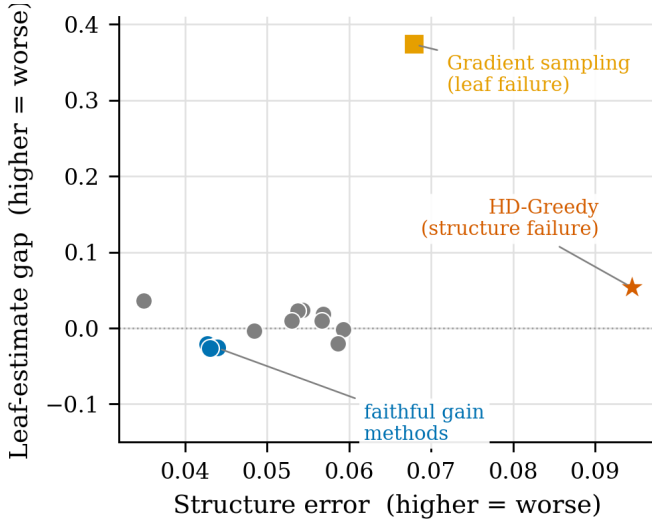
Fig. 5: Two failure modes. HD-Greedy is structure-dominated; gradient sampling is leaf-estimate dominated. Faithful gain methods occupy the low-error corner.
