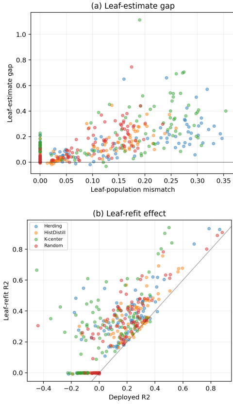
Fig. 9: Regression decomposition. Structure loss dominates for every method; leaf refitting helps modestly but does not close the gap to the structure reference.
