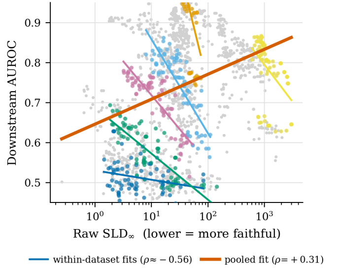
Fig. 3: Within-dataset SLD trend. Coloured lines are within-dataset fits on log-scale raw SLD; the average within-dataset trend is negative. The bold orange pooled fit reverses because dataset scale confounds raw SLD and AUROC.
