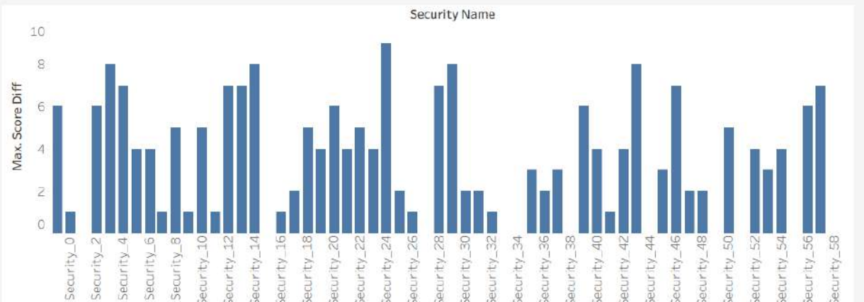
Top Outliers
