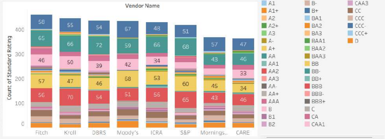
Top Outliers
