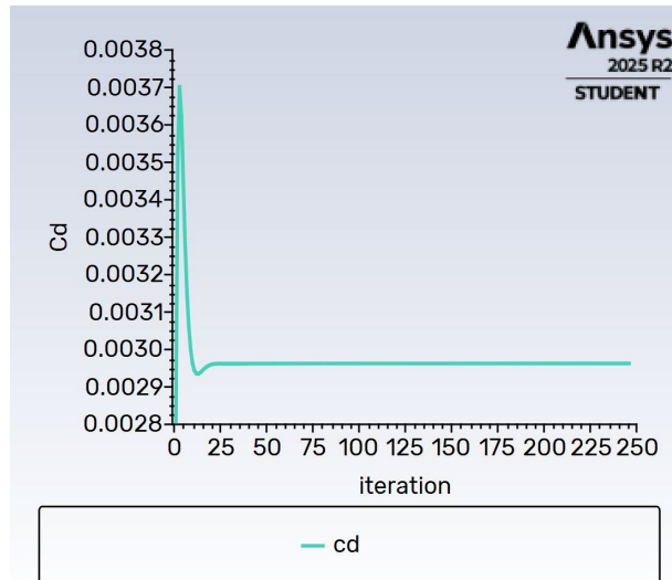
Figure 8b. Drag coefficient, 0^\circ AOA.
