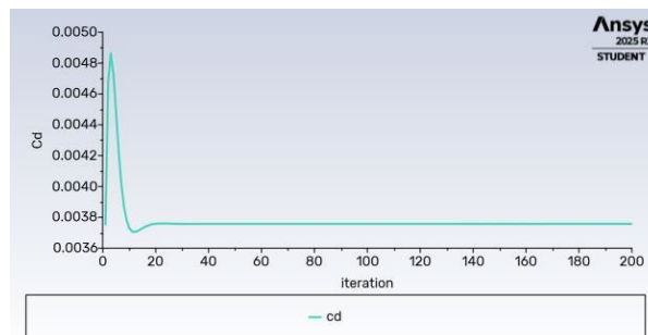
Figure 7b. Drag coefficient, -2° AOA.
