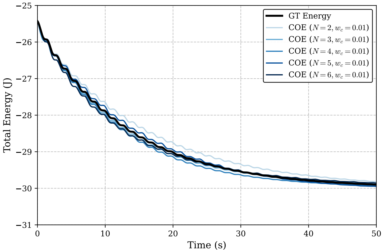
Total Energy (50.0s Rollout) - Scaling N at w_c = 0.01
